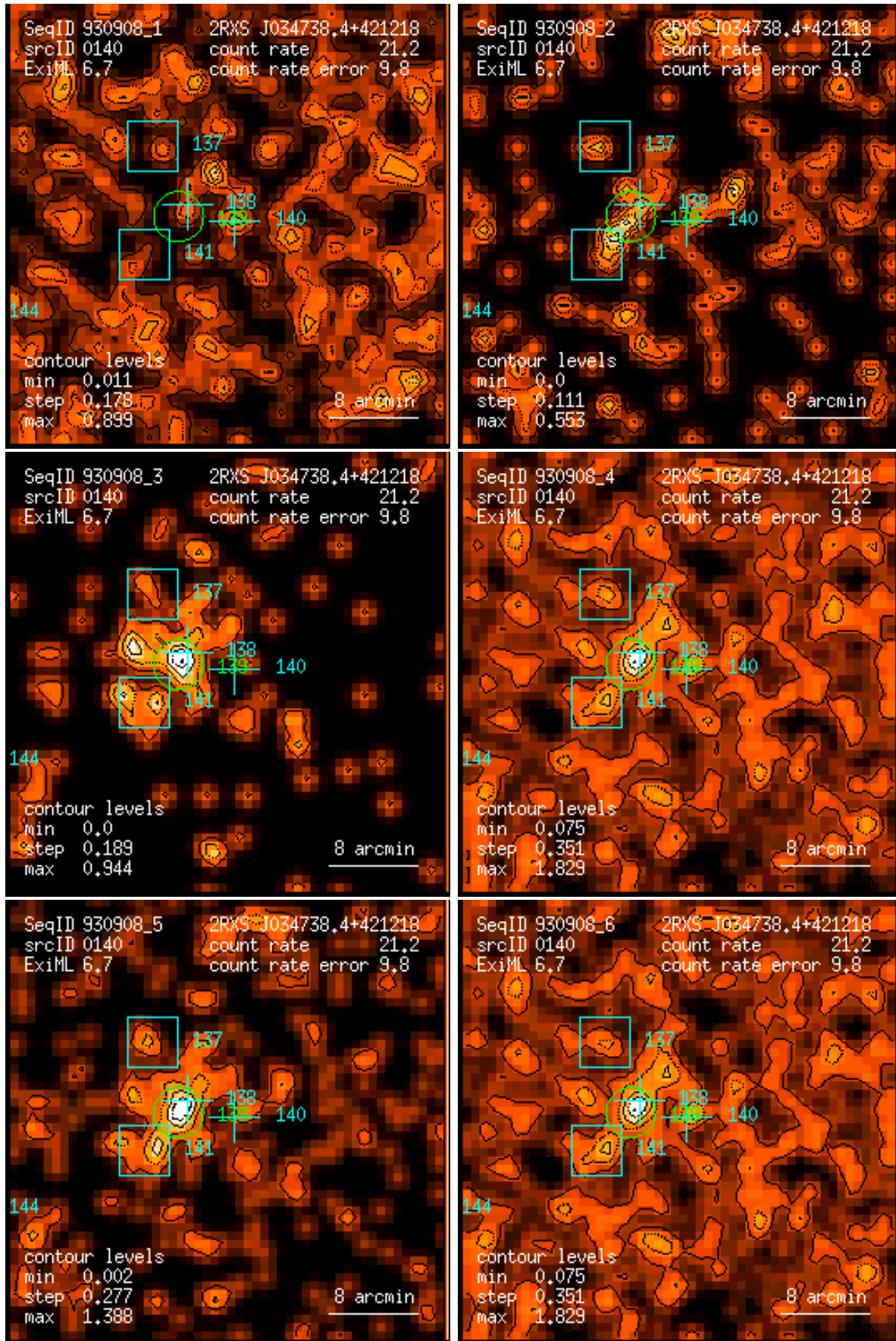
Figure 140: RASS 930908: detection 0140: band rate images, Gaussian filter: (1) PSPC channels 11 – 41, (2) 52 – 90, (3) 91 – 201, (4) 11 – 235, (5) 52 – 201, (6) 11 – 201. Broad band rates in counts/ks. Band rate contour levels in counts/ks/arcmin 2 .
