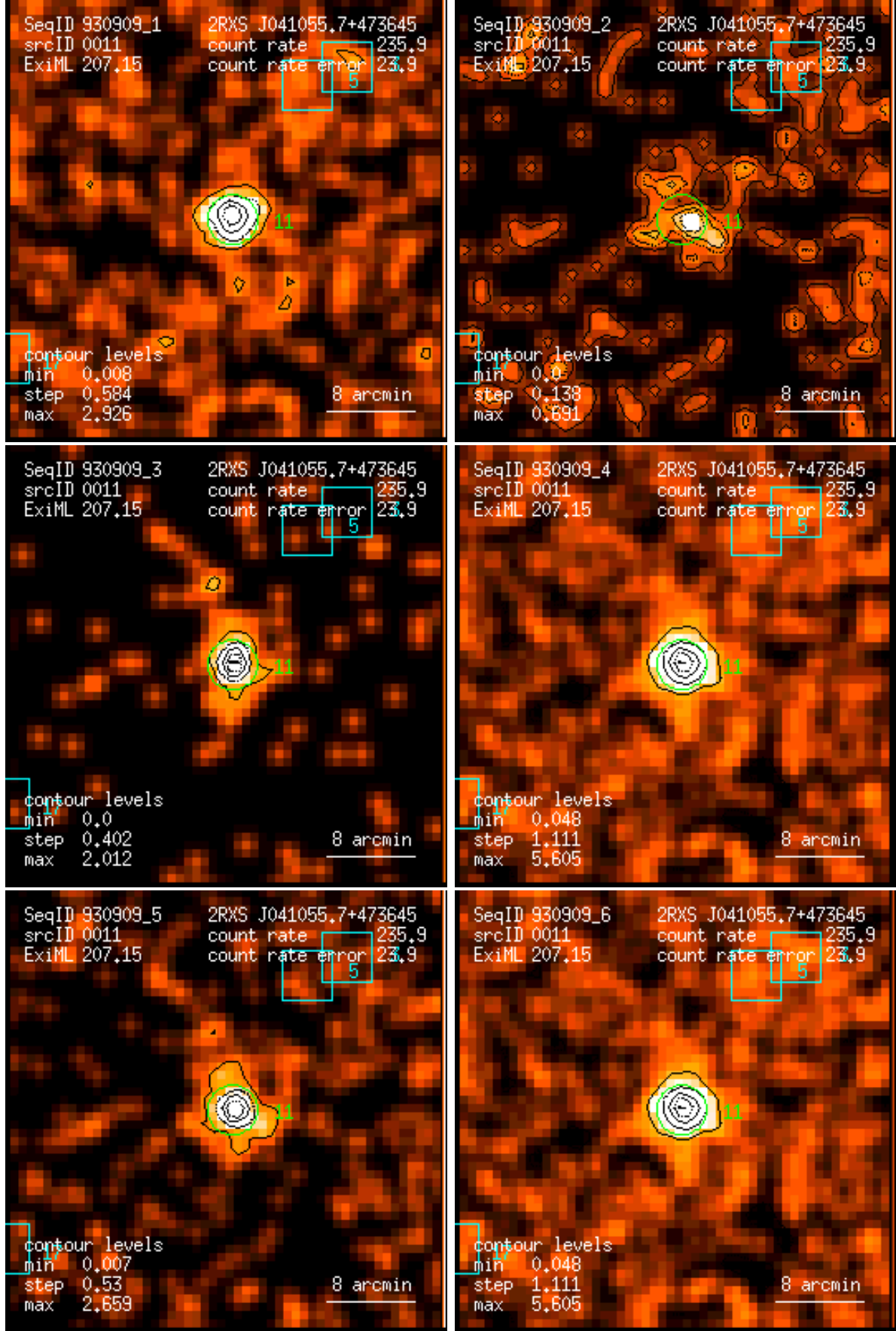
Figure 11: RASS 930909: detection 0011: band rate images, Gaussian filter: (1) PSPC channels 11 – 41, (2) 52 – 90, (3) 91 – 201, (4) 11 – 235, (5) 52 – 201, (6) 11 – 201. Broad band rates in counts/ks. Band rate contour levels in counts/ks/arcmin 2 .
