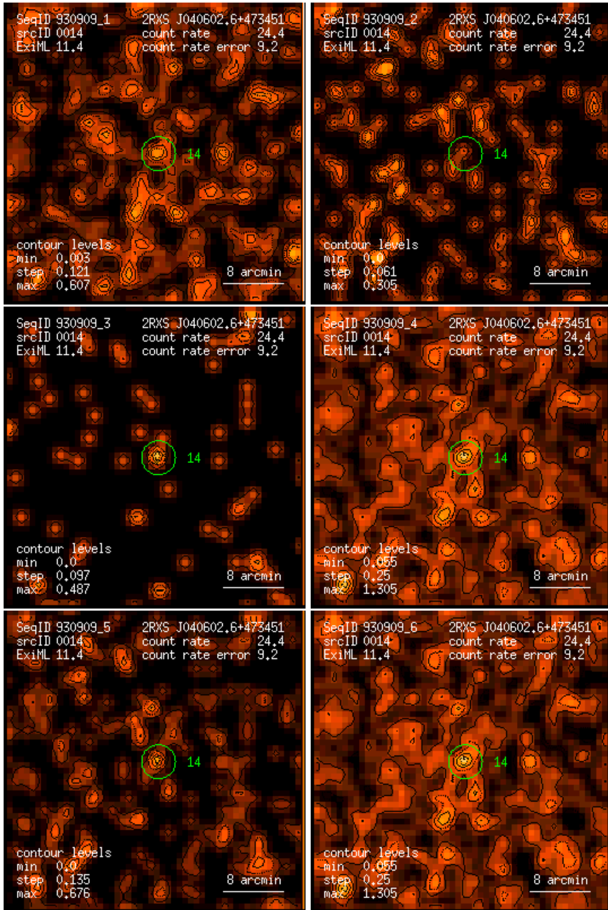
Figure 14: RASS 930909: detection 0014: band rate images, Gaussian filter: (1) PSPC channels 11 – 41, (2) 52 – 90, (3) 91 – 201, (4) 11 – 235, (5) 52 – 201, (6) 11 – 201. Broad band rates in counts/ks. Band rate contour levels in counts/ks/arcmin 2 .
