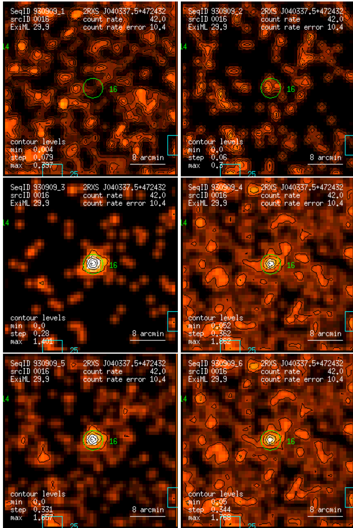
Figure 16: RASS 930909: detection 0016: band rate images, Gaussian filter: (1) PSPC channels 11 – 41, (2) 52 – 90, (3) 91 – 201, (4) 11 – 235, (5) 52 – 201, (6) 11 – 201. Broad band rates in counts/ks. Band rate contour levels in counts/ks/arcmin 2 .
