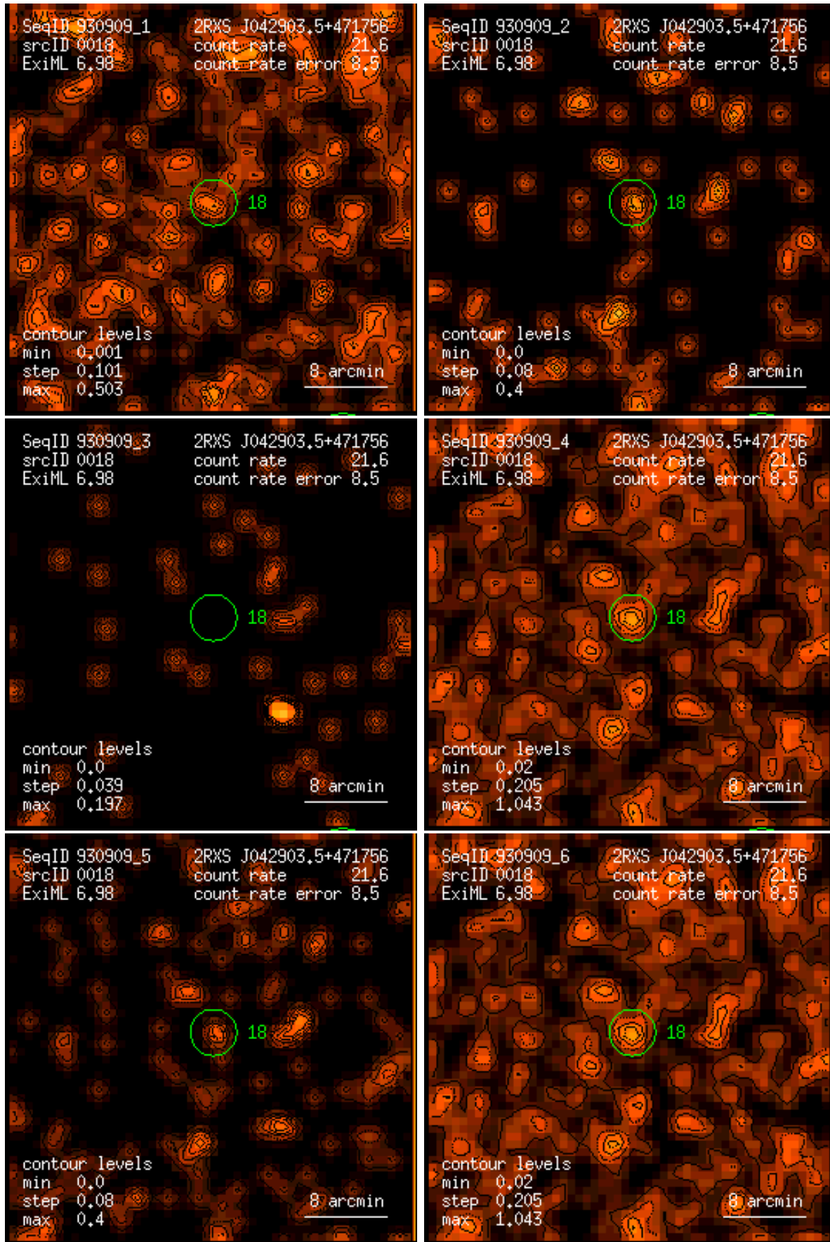
Figure 18: RASS 930909: detection 0018: band rate images, Gaussian filter: (1) PSPC channels 11 – 41, (2) 52 – 90, (3) 91 – 201, (4) 11 – 235, (5) 52 – 201, (6) 11 – 201. Broad band rates in counts/ks. Band rate contour levels in counts/ks/arcmin 2 .
