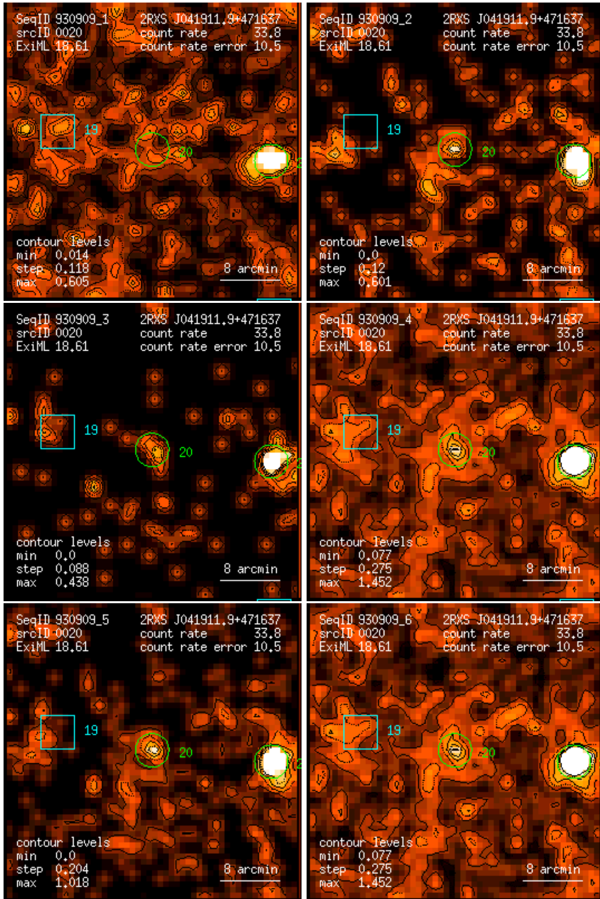
Figure 20: RASS 930909: detection 0020: band rate images, Gaussian filter: (1) PSPC channels 11 – 41, (2) 52 – 90, (3) 91 – 201, (4) 11 – 235, (5) 52 – 201, (6) 11 – 201. Broad band rates in counts/ks. Band rate contour levels in counts/ks/arcmin 2 .
