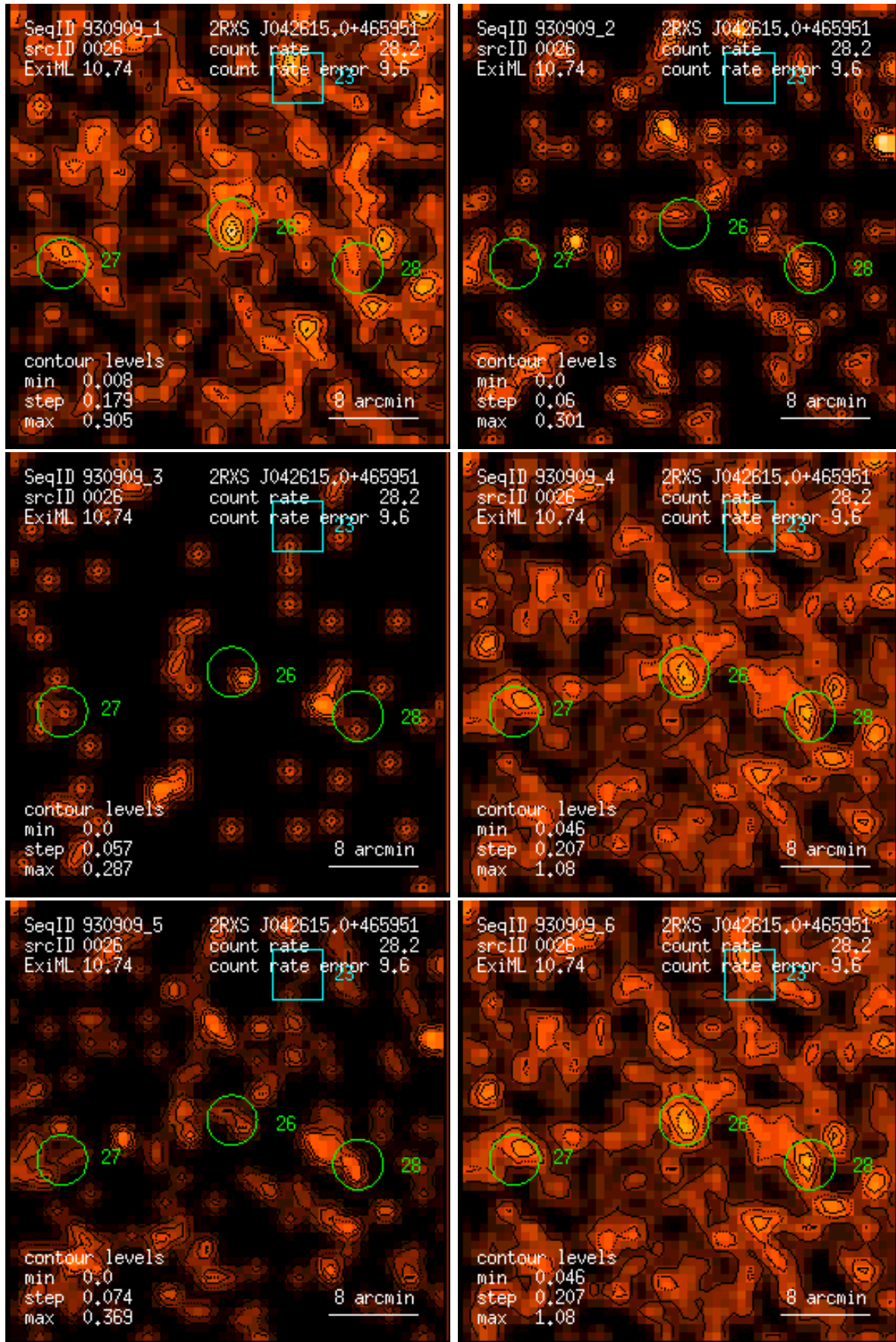
Figure 26: RASS 930909: detection 0026: band rate images, Gaussian filter: (1) PSPC channels 11 – 41, (2) 52 – 90, (3) 91 – 201, (4) 11 – 235, (5) 52 – 201, (6) 11 – 201. Broad band rates in counts/ks. Band rate contour levels in counts/ks/arcmin 2 .
