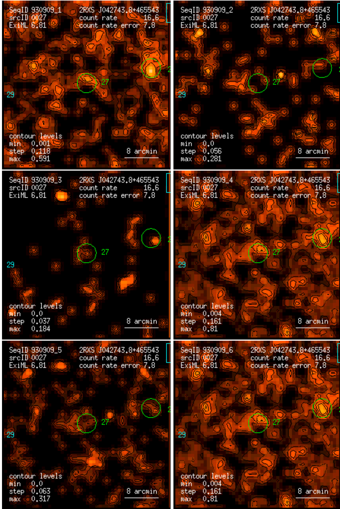
Figure 27: RASS 930909: detection 0027: band rate images, Gaussian filter: (1) PSPC channels 11 – 41, (2) 52 – 90, (3) 91 – 201, (4) 11 – 235, (5) 52 – 201, (6) 11 – 201. Broad band rates in counts/ks. Band rate contour levels in counts/ks/arcmin 2 .
