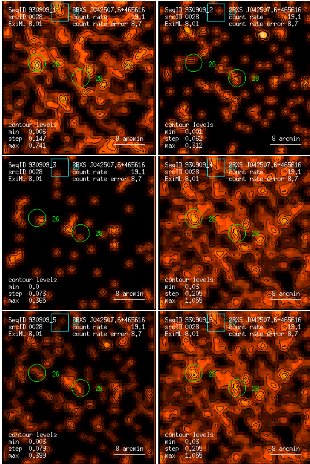
Figure 28: RASS 930909: detection 0028: band rate images, Gaussian filter: (1) PSPC channels 11 – 41, (2) 52 – 90, (3) 91 – 201, (4) 11 – 235, (5) 52 – 201, (6) 11 – 201. Broad band rates in counts/ks. Band rate contour levels in counts/ks/arcmin 2 .
