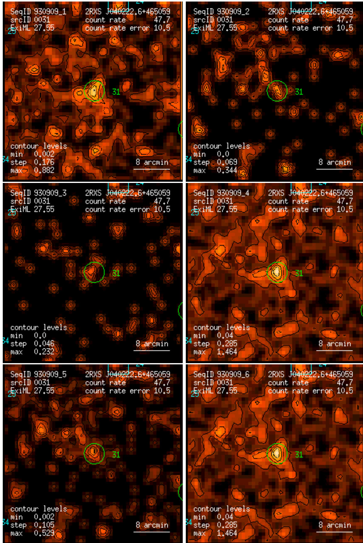
Figure 31: RASS 930909: detection 0031: band rate images, Gaussian filter: (1) PSPC channels 11 – 41, (2) 52 – 90, (3) 91 – 201, (4) 11 – 235, (5) 52 – 201, (6) 11 – 201. Broad band rates in counts/ks. Band rate contour levels in counts/ks/arcmin 2 .
