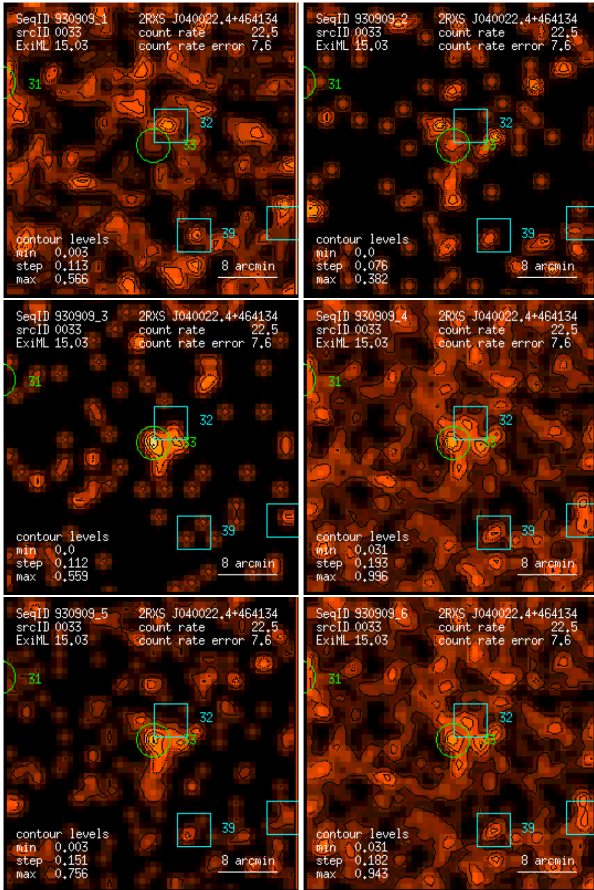
Figure 33: RASS 930909: detection 0033: band rate images, Gaussian filter: (1) PSPC channels 11 – 41, (2) 52 – 90, (3) 91 – 201, (4) 11 – 235, (5) 52 – 201, (6) 11 – 201. Broad band rates in counts/ks. Band rate contour levels in counts/ks/arcmin 2 .
