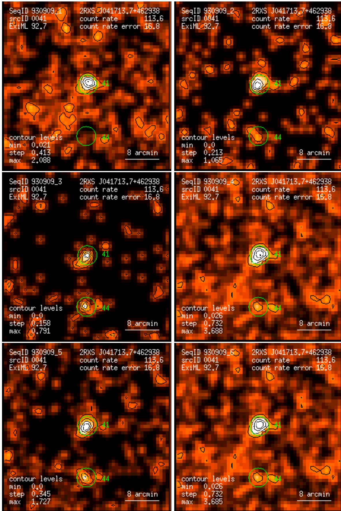
Figure 41: RASS 930909: detection 0041: band rate images, Gaussian filter: (1) PSPC channels 11 – 41, (2) 52 – 90, (3) 91 – 201, (4) 11 – 235, (5) 52 – 201, (6) 11 – 201. Broad band rates in counts/ks. Band rate contour levels in counts/ks/arcmin 2 .
