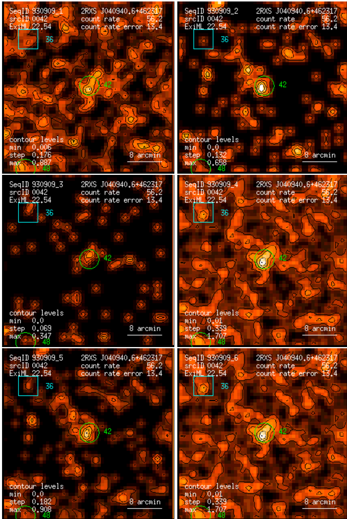
Figure 42: RASS 930909: detection 0042: band rate images, Gaussian filter: (1) PSPC channels 11 – 41, (2) 52 – 90, (3) 91 – 201, (4) 11 – 235, (5) 52 – 201, (6) 11 – 201. Broad band rates in counts/ks. Band rate contour levels in counts/ks/arcmin 2 .
