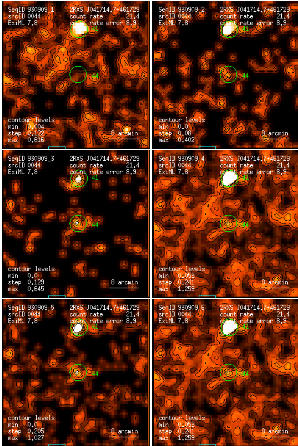
Figure 44: RASS 930909: detection 0044: band rate images, Gaussian filter: (1) PSPC channels 11 – 41, (2) 52 – 90, (3) 91 – 201, (4) 11 – 235, (5) 52 – 201, (6) 11 – 201. Broad band rates in counts/ks. Band rate contour levels in counts/ks/arcmin 2 .
