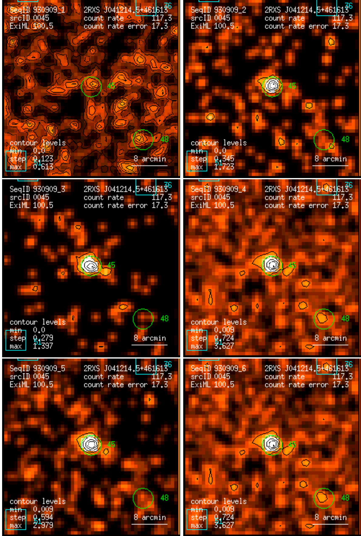
Figure 45: RASS 930909: detection 0045: band rate images, Gaussian filter: (1) PSPC channels 11 – 41, (2) 52 – 90, (3) 91 – 201, (4) 11 – 235, (5) 52 – 201, (6) 11 – 201. Broad band rates in counts/ks. Band rate contour levels in counts/ks/arcmin 2 .
