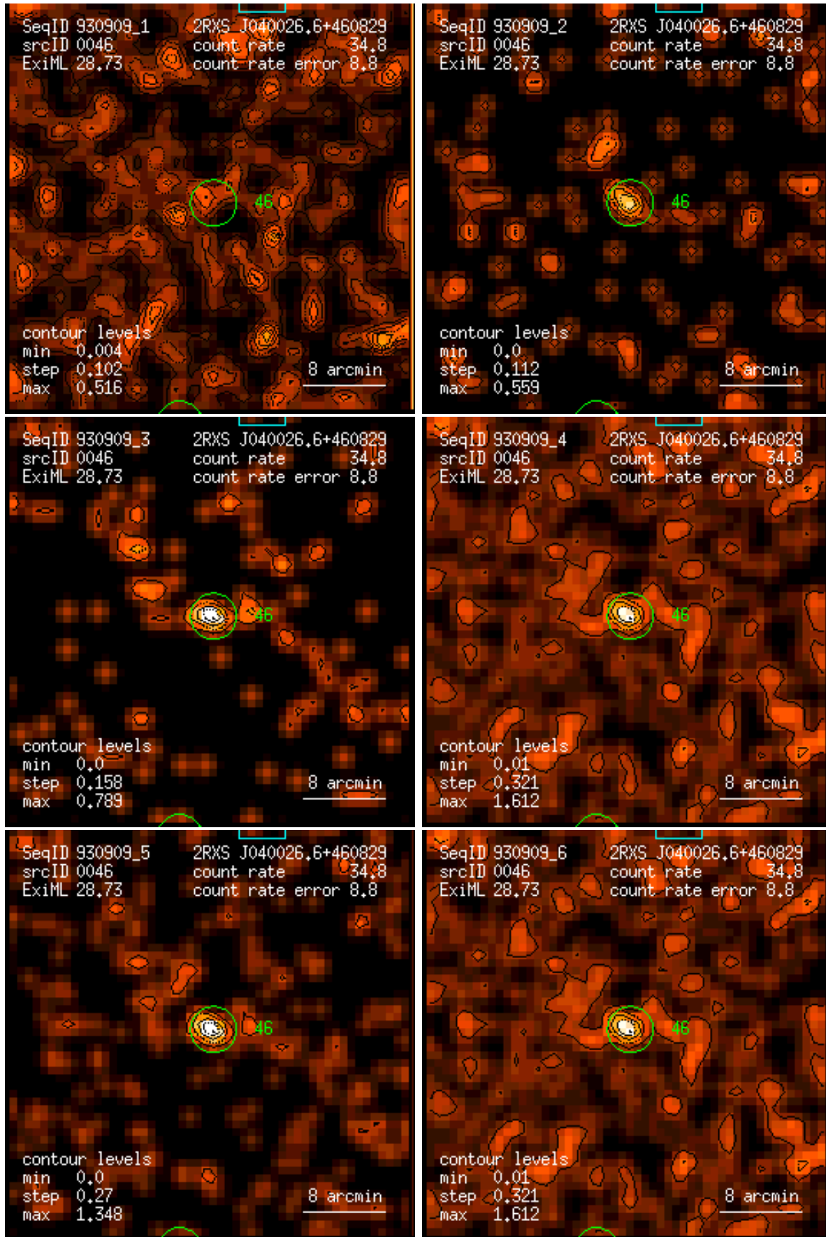
Figure 46: RASS 930909: detection 0046: band rate images, Gaussian filter: (1) PSPC channels 11 – 41, (2) 52 – 90, (3) 91 – 201, (4) 11 – 235, (5) 52 – 201, (6) 11 – 201. Broad band rates in counts/ks. Band rate contour levels in counts/ks/arcmin 2 .
