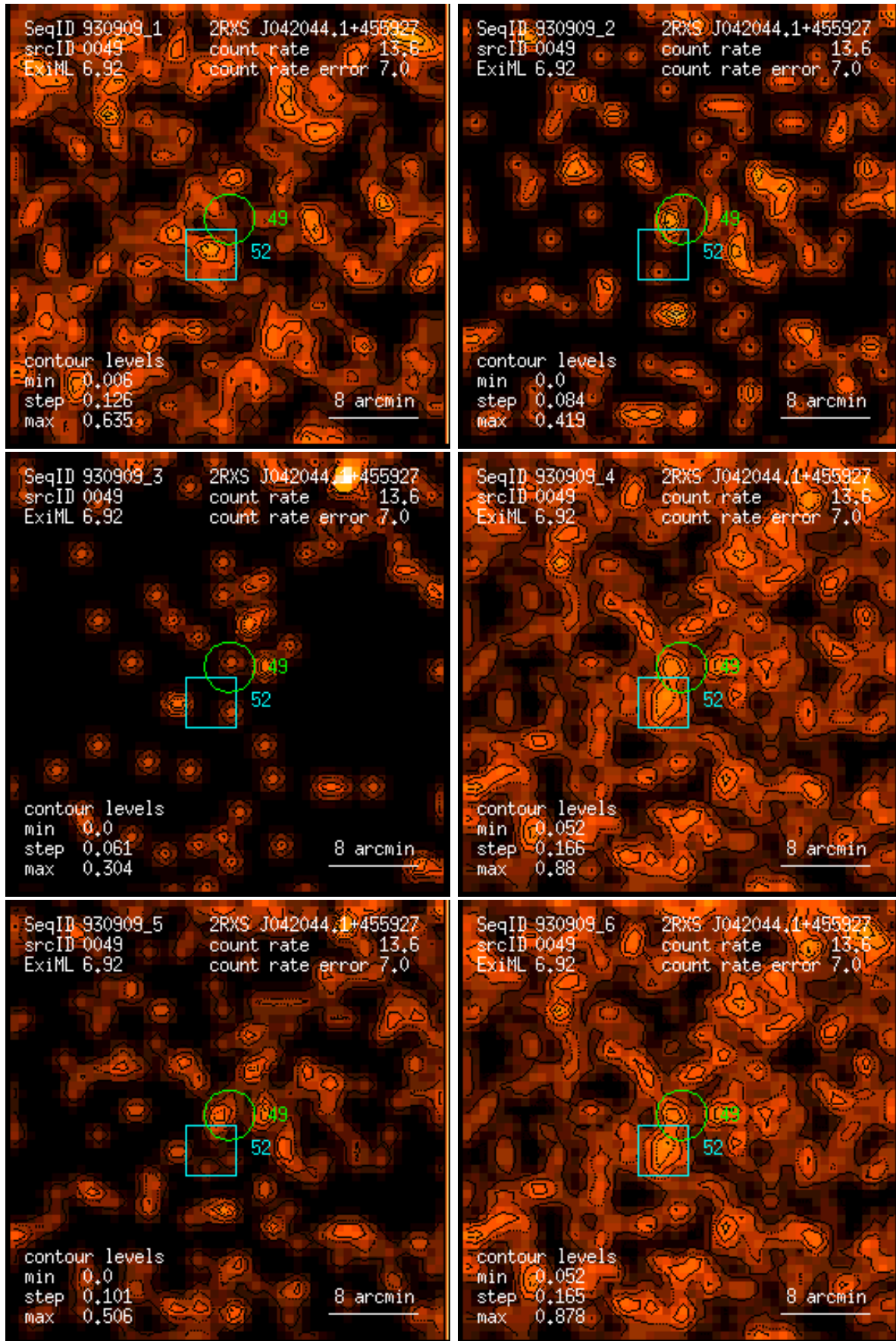
Figure 49: RASS 930909: detection 0049: band rate images, Gaussian filter: (1) PSPC channels 11 – 41, (2) 52 – 90, (3) 91 – 201, (4) 11 – 235, (5) 52 – 201, (6) 11 – 201. Broad band rates in counts/ks. Band rate contour levels in counts/ks/arcmin 2 .
