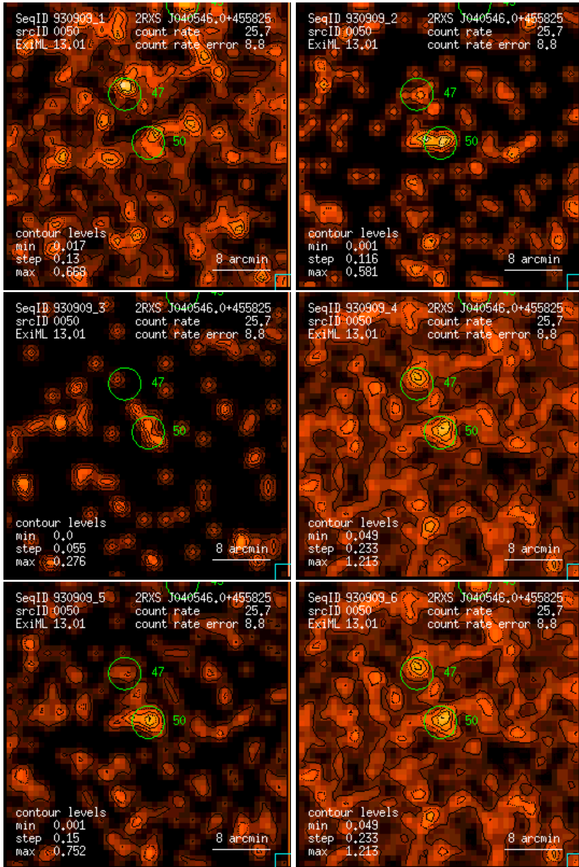
Figure 50: RASS 930909: detection 0050: band rate images, Gaussian filter: (1) PSPC channels 11 – 41, (2) 52 – 90, (3) 91 – 201, (4) 11 – 235, (5) 52 – 201, (6) 11 – 201. Broad band rates in counts/ks. Band rate contour levels in counts/ks/arcmin 2 .
