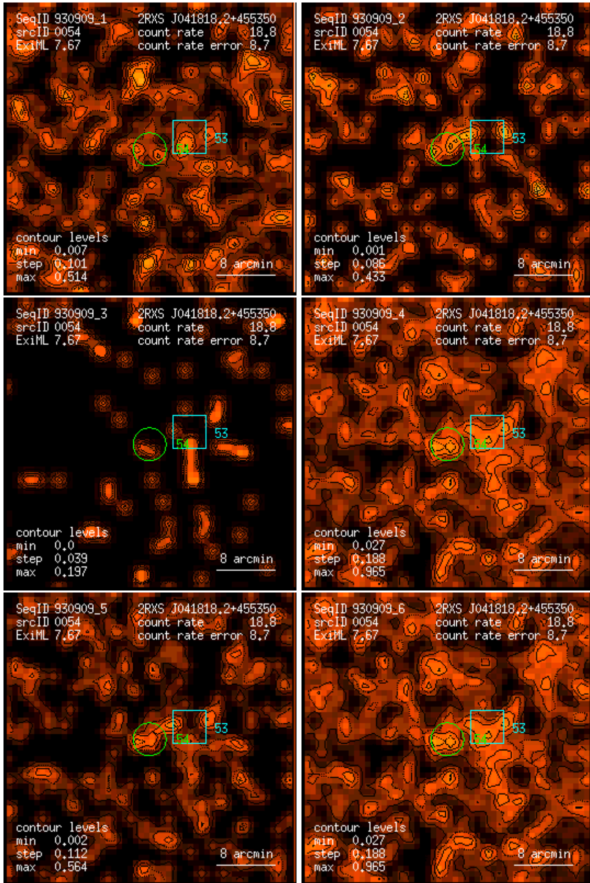
Figure 54: RASS 930909: detection 0054: band rate images, Gaussian filter: (1) PSPC channels 11 – 41, (2) 52 – 90, (3) 91 – 201, (4) 11 – 235, (5) 52 – 201, (6) 11 – 201. Broad band rates in counts/ks. Band rate contour levels in counts/ks/arcmin 2 .
