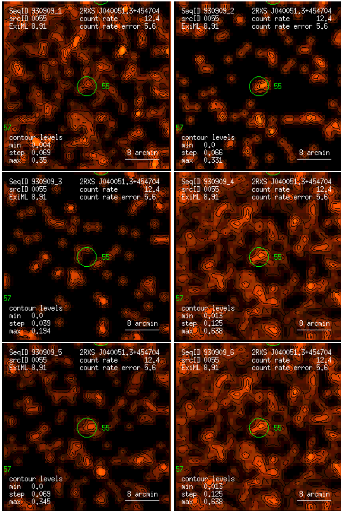
Figure 55: RASS 930909: detection 0055: band rate images, Gaussian filter: (1) PSPC channels 11 – 41, (2) 52 – 90, (3) 91 – 201, (4) 11 – 235, (5) 52 – 201, (6) 11 – 201. Broad band rates in counts/ks. Band rate contour levels in counts/ks/arcmin 2 .
