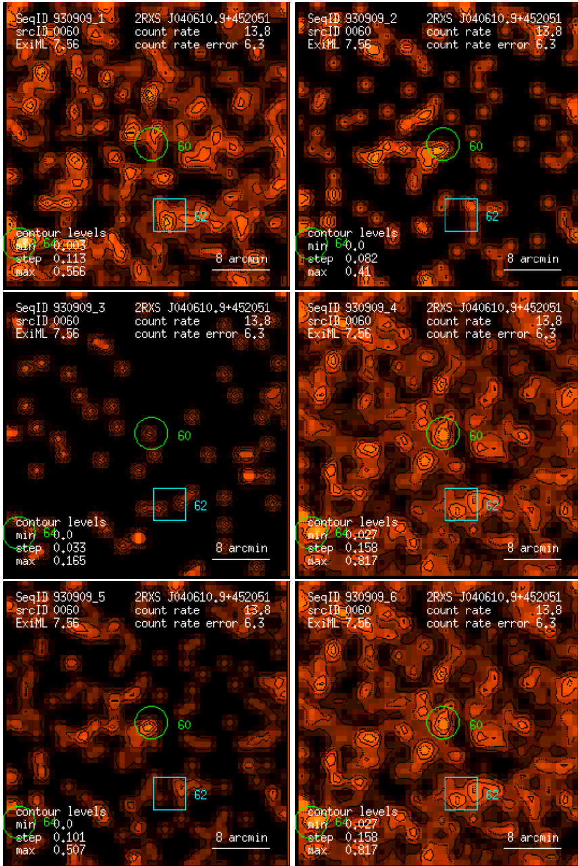
Figure 60: RASS 930909: detection 0060: band rate images, Gaussian filter: (1) PSPC channels 11 – 41, (2) 52 – 90, (3) 91 – 201, (4) 11 – 235, (5) 52 – 201, (6) 11 – 201. Broad band rates in counts/ks. Band rate contour levels in counts/ks/arcmin 2 .
