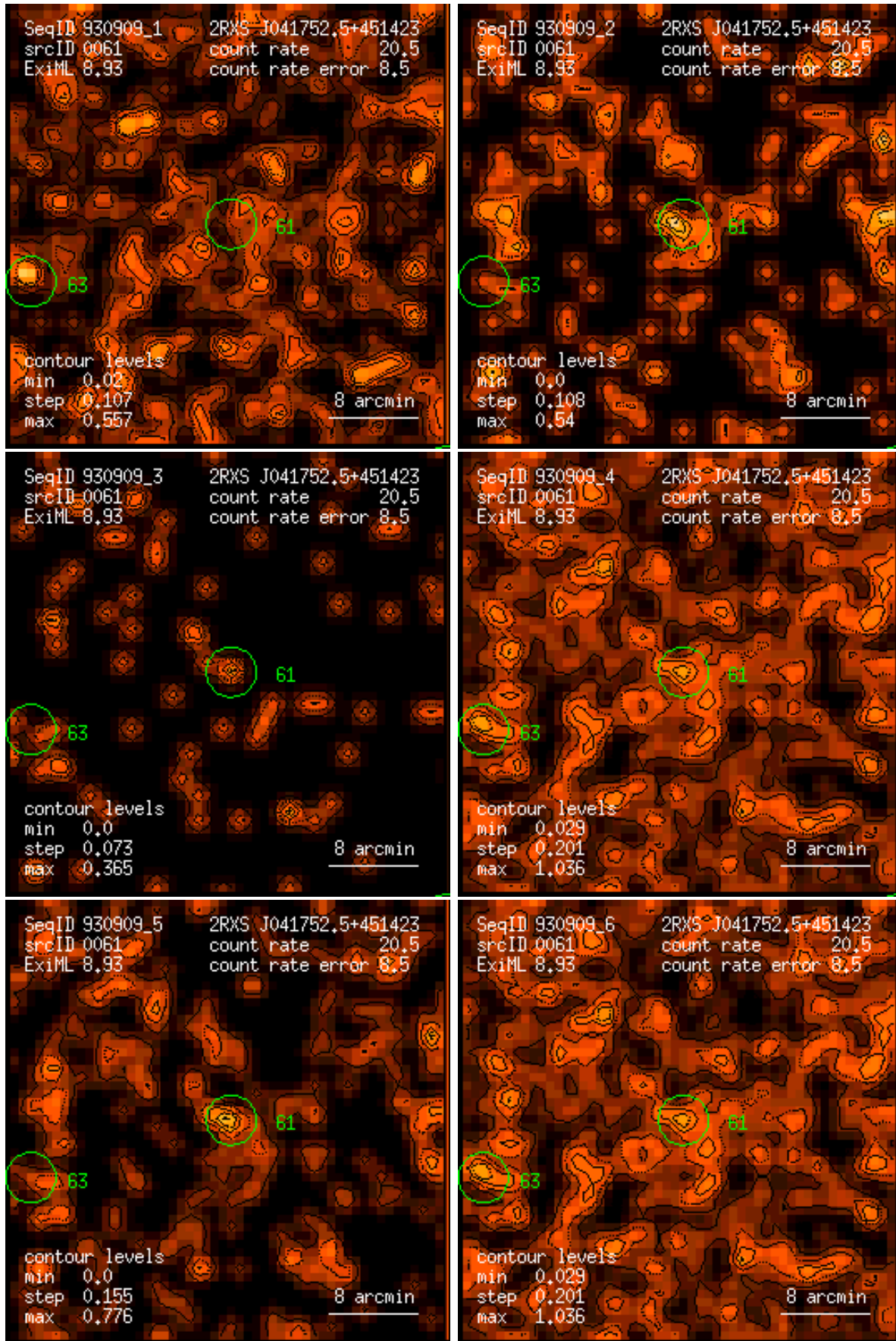
Figure 61: RASS 930909: detection 0061: band rate images, Gaussian filter: (1) PSPC channels 11 – 41, (2) 52 – 90, (3) 91 – 201, (4) 11 – 235, (5) 52 – 201, (6) 11 – 201. Broad band rates in counts/ks. Band rate contour levels in counts/ks/arcmin 2 .
