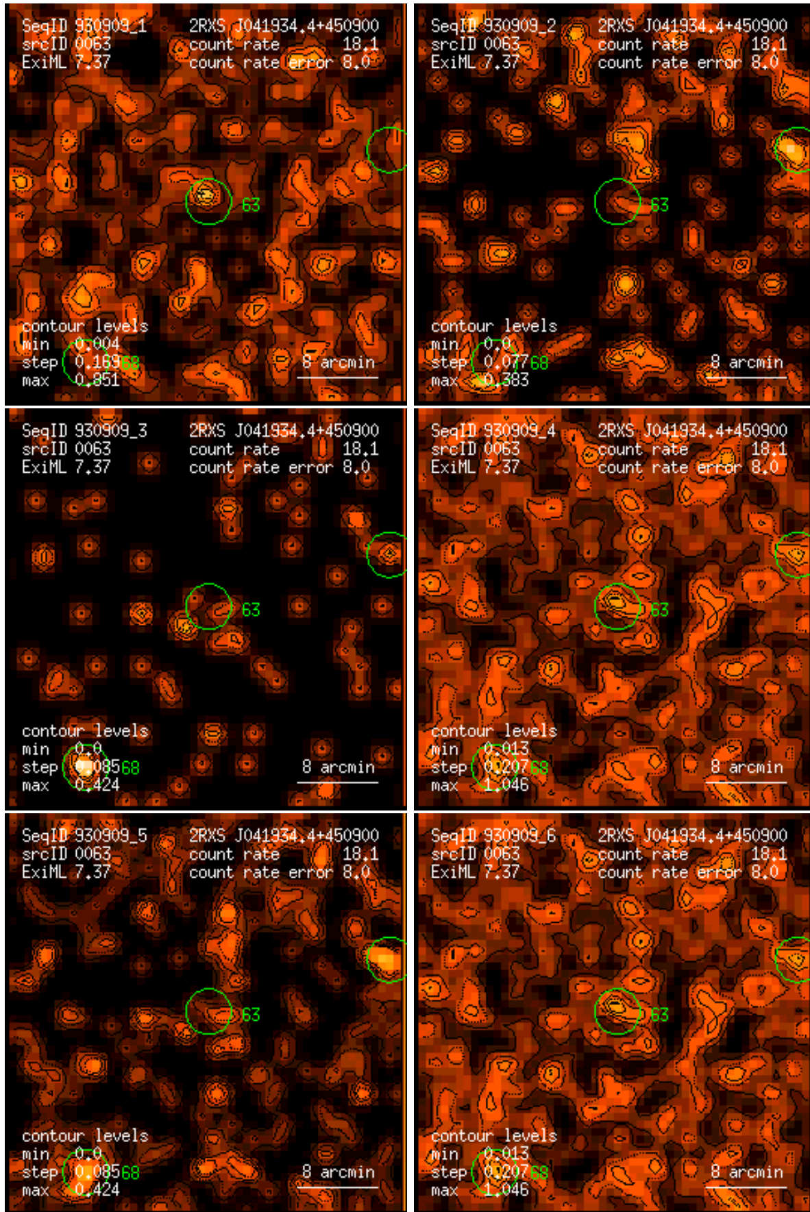
Figure 63: RASS 930909: detection 0063: band rate images, Gaussian filter: (1) PSPC channels 11 – 41, (2) 52 – 90, (3) 91 – 201, (4) 11 – 235, (5) 52 – 201, (6) 11 – 201. Broad band rates in counts/ks. Band rate contour levels in counts/ks/arcmin 2 .
