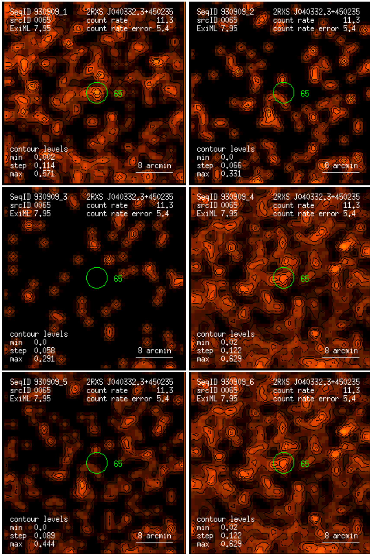
Figure 65: RASS 930909: detection 0065: band rate images, Gaussian filter: (1) PSPC channels 11 – 41, (2) 52 – 90, (3) 91 – 201, (4) 11 – 235, (5) 52 – 201, (6) 11 – 201. Broad band rates in counts/ks. Band rate contour levels in counts/ks/arcmin 2 .
