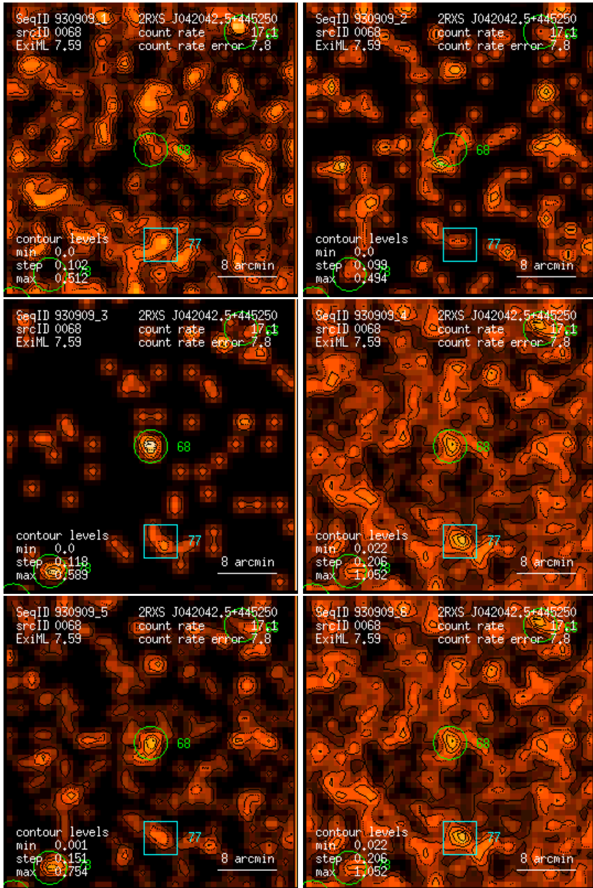
Figure 68: RASS 930909: detection 0068: band rate images, Gaussian filter: (1) PSPC channels 11 – 41, (2) 52 – 90, (3) 91 – 201, (4) 11 – 235, (5) 52 – 201, (6) 11 – 201. Broad band rates in counts/ks. Band rate contour levels in counts/ks/arcmin 2 .
