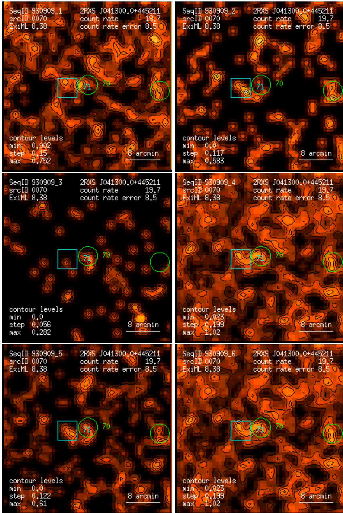
Figure 70: RASS 930909: detection 0070: band rate images, Gaussian filter: (1) PSPC channels 11 – 41, (2) 52 – 90, (3) 91 – 201, (4) 11 – 235, (5) 52 – 201, (6) 11 – 201. Broad band rates in counts/ks. Band rate contour levels in counts/ks/arcmin 2 .
