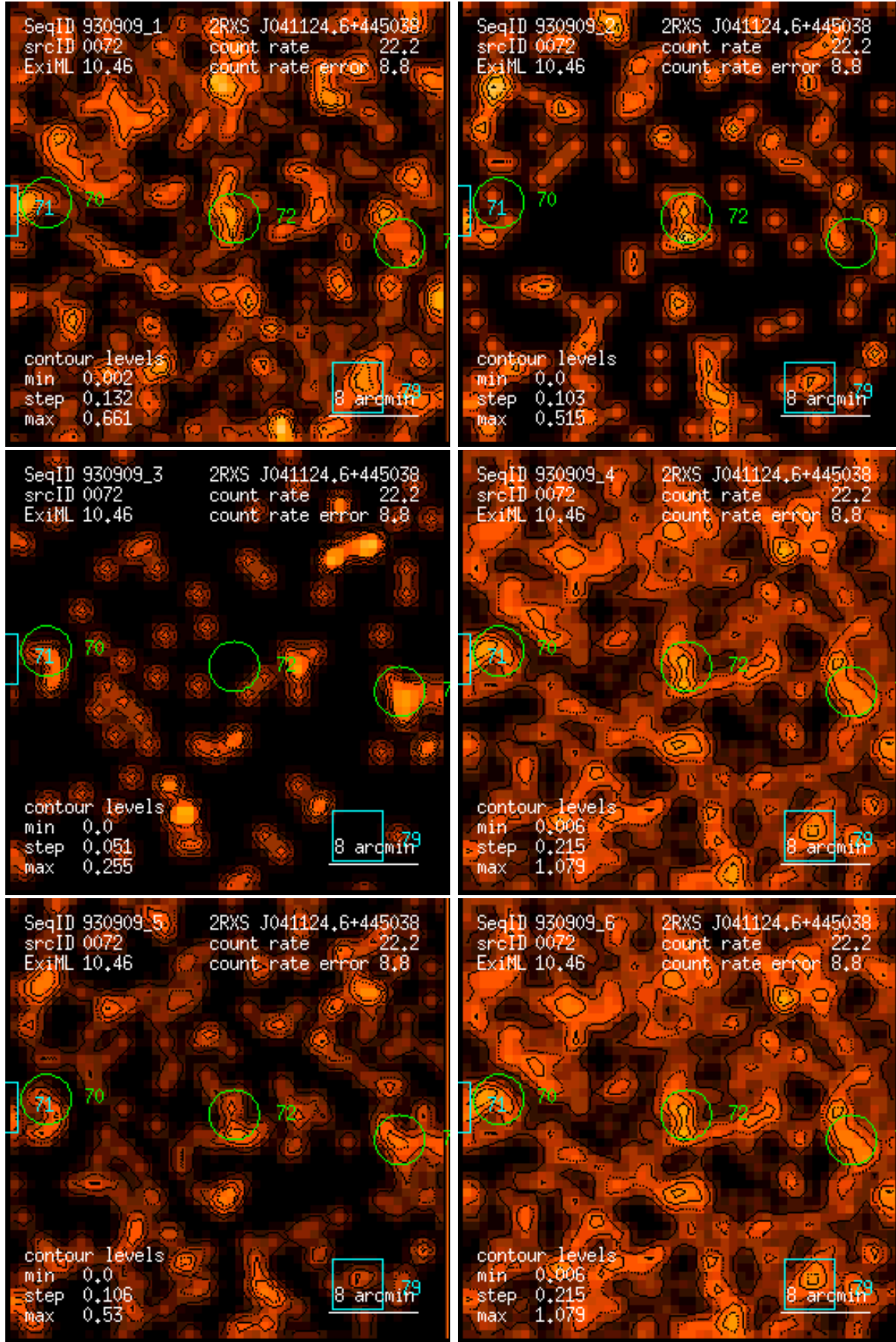
Figure 72: RASS 930909: detection 0072: band rate images, Gaussian filter: (1) PSPC channels 11 – 41, (2) 52 – 90, (3) 91 – 201, (4) 11 – 235, (5) 52 – 201, (6) 11 – 201. Broad band rates in counts/ks. Band rate contour levels in counts/ks/arcmin 2 .
