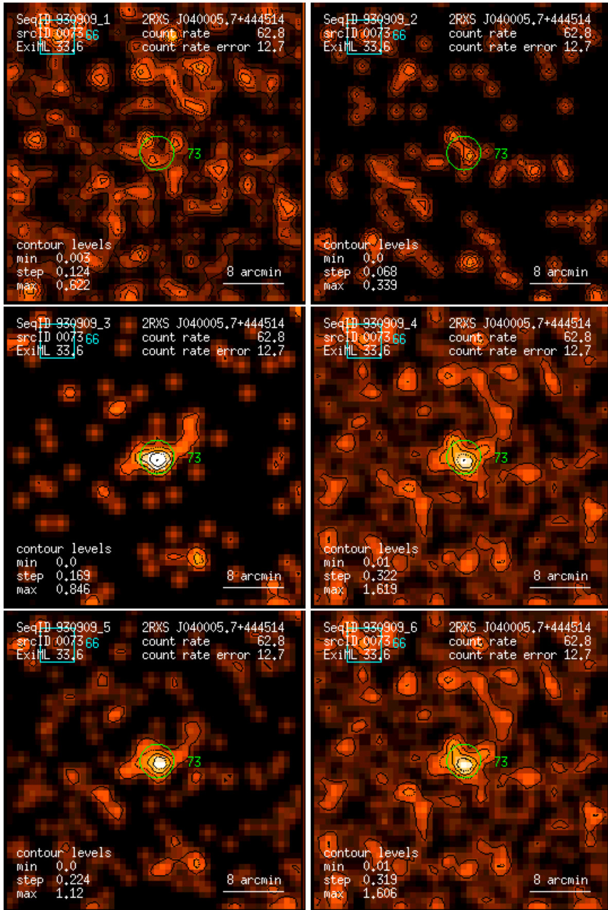
Figure 73: RASS 930909: detection 0073: band rate images, Gaussian filter: (1) PSPC channels 11 – 41, (2) 52 – 90, (3) 91 – 201, (4) 11 – 235, (5) 52 – 201, (6) 11 – 201. Broad band rates in counts/ks. Band rate contour levels in counts/ks/arcmin 2 .
