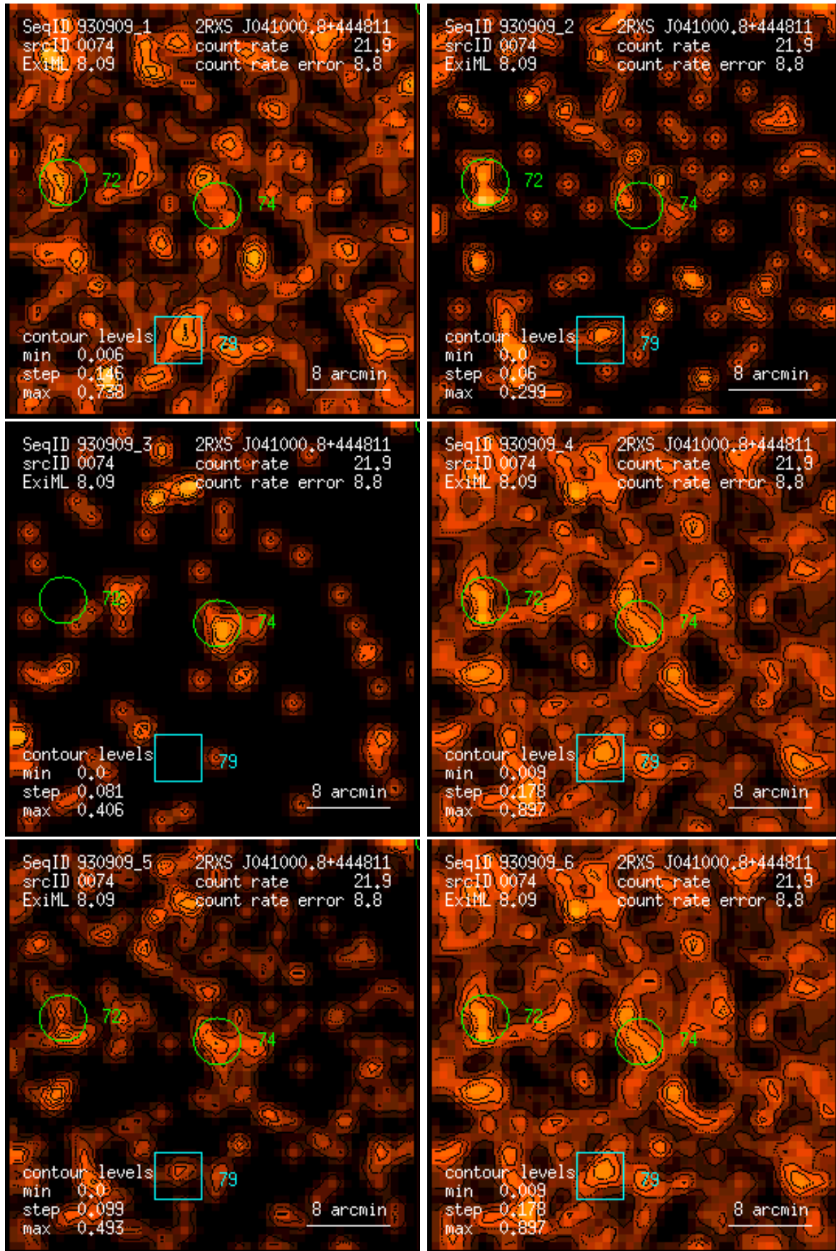
Figure 74: RASS 930909: detection 0074: band rate images, Gaussian filter: (1) PSPC channels 11 – 41, (2) 52 – 90, (3) 91 – 201, (4) 11 – 235, (5) 52 – 201, (6) 11 – 201. Broad band rates in counts/ks. Band rate contour levels in counts/ks/arcmin 2 .
