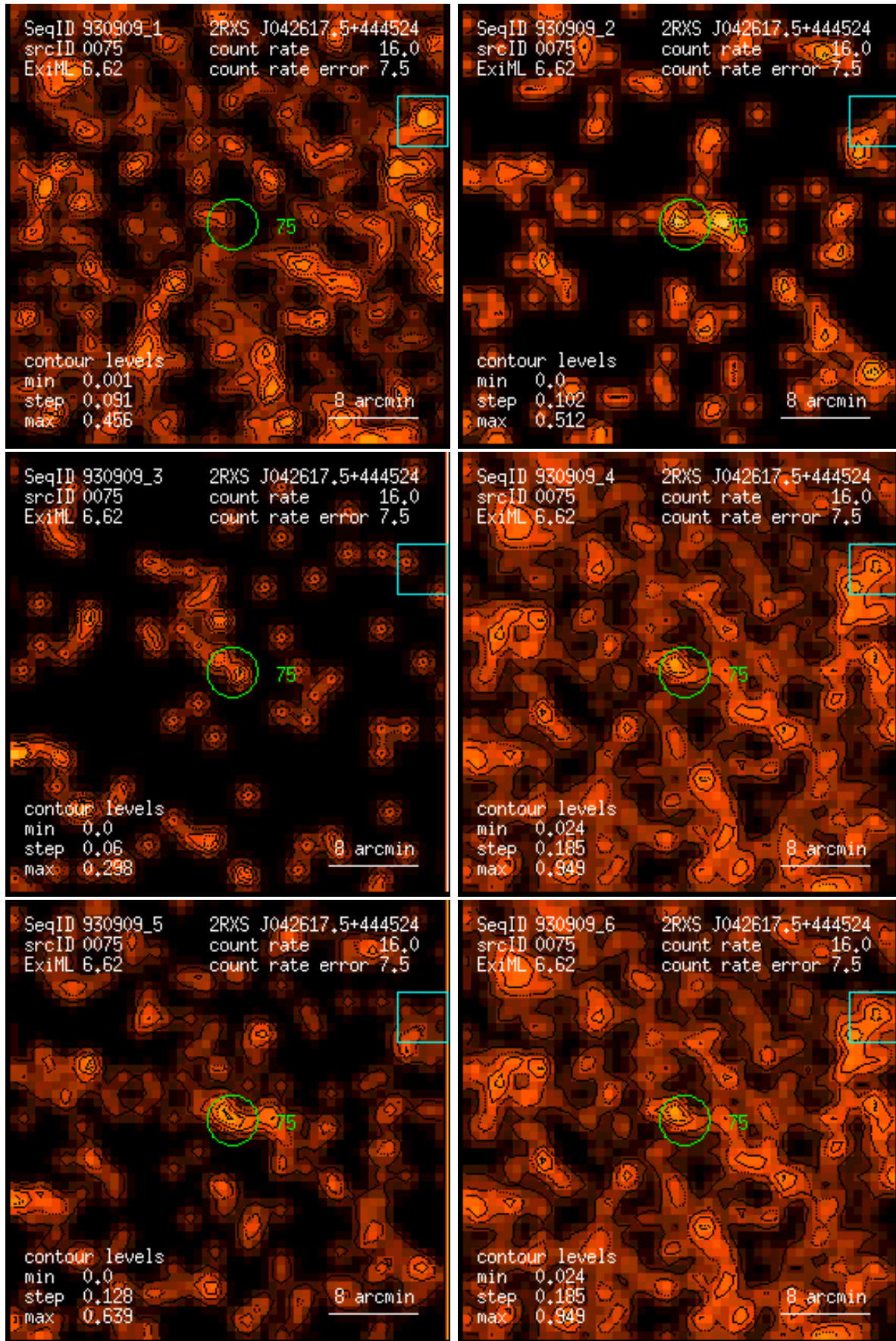
Figure 75: RASS 930909: detection 0075: band rate images, Gaussian filter: (1) PSPC channels 11 – 41, (2) 52 – 90, (3) 91 – 201, (4) 11 – 235, (5) 52 – 201, (6) 11 – 201. Broad band rates in counts/ks. Band rate contour levels in counts/ks/arcmin 2 .
