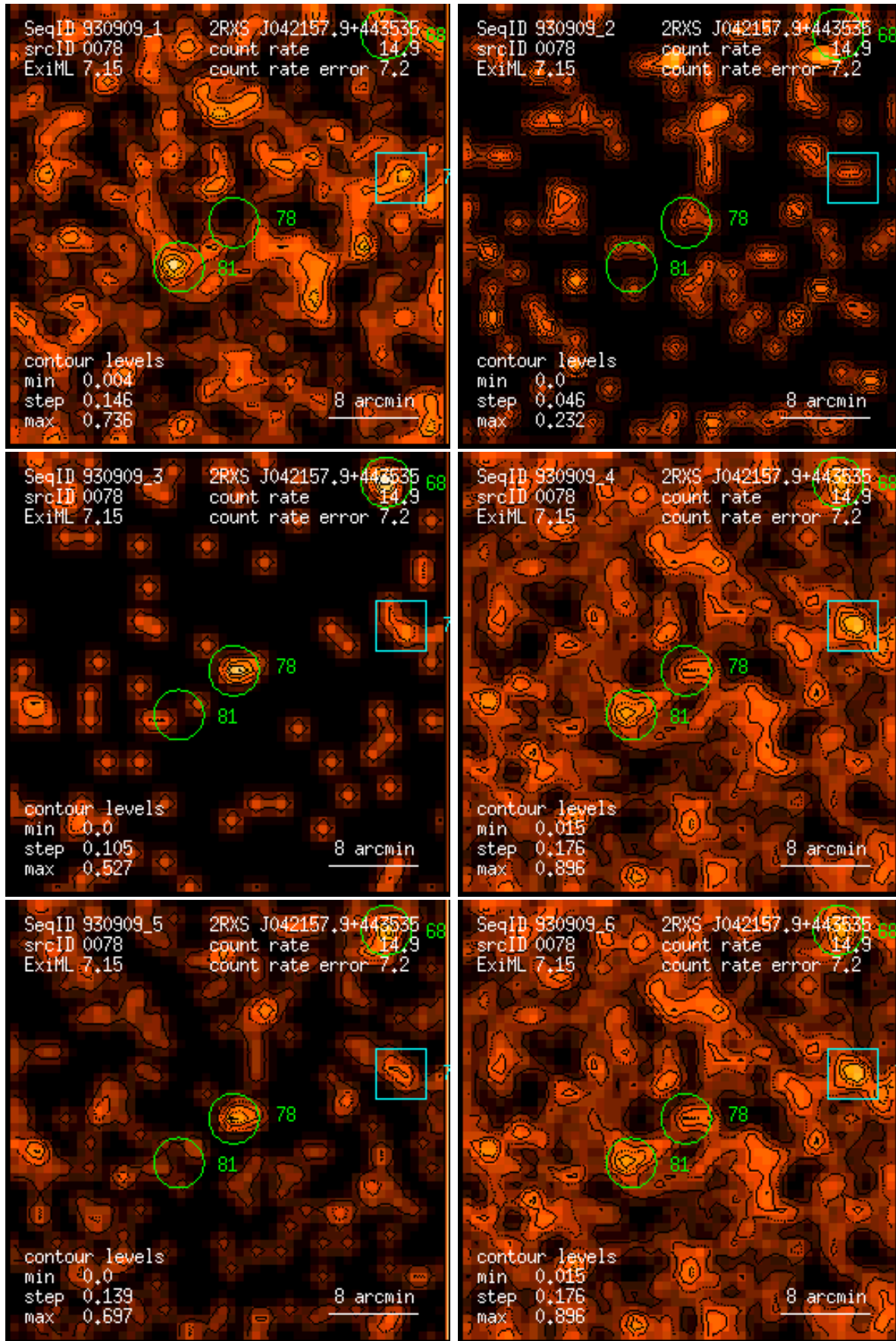
Figure 78: RASS 930909: detection 0078: band rate images, Gaussian filter: (1) PSPC channels 11 – 41, (2) 52 – 90, (3) 91 – 201, (4) 11 – 235, (5) 52 – 201, (6) 11 – 201. Broad band rates in counts/ks. Band rate contour levels in counts/ks/arcmin 2 .
