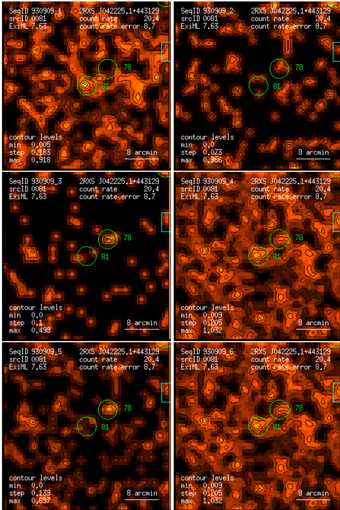
Figure 81: RASS 930909: detection 0081: band rate images, Gaussian filter: (1) PSPC channels 11 – 41, (2) 52 – 90, (3) 91 – 201, (4) 11 – 235, (5) 52 – 201, (6) 11 – 201. Broad band rates in counts/ks. Band rate contour levels in counts/ks/arcmin 2 .
