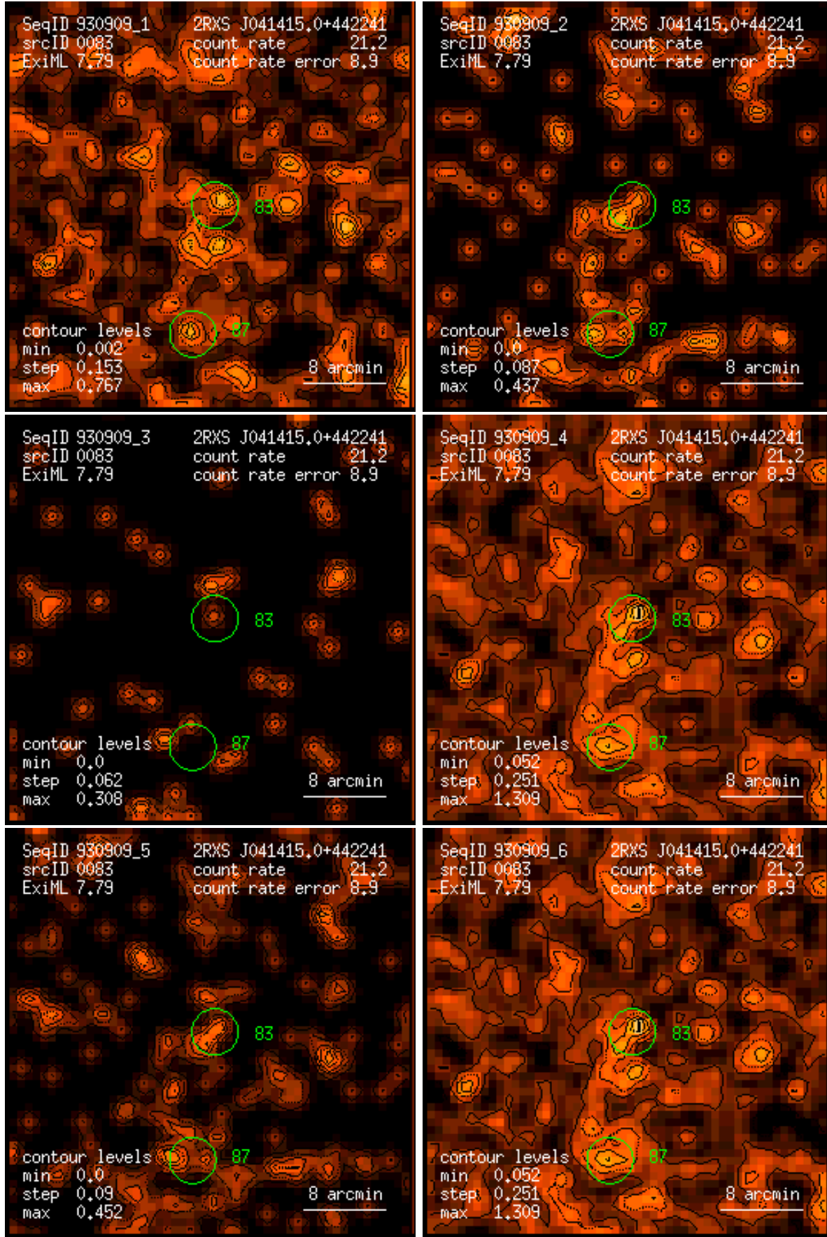
Figure 83: RASS 930909: detection 0083: band rate images, Gaussian filter: (1) PSPC channels 11 – 41, (2) 52 – 90, (3) 91 – 201, (4) 11 – 235, (5) 52 – 201, (6) 11 – 201. Broad band rates in counts/ks. Band rate contour levels in counts/ks/arcmin 2 .
