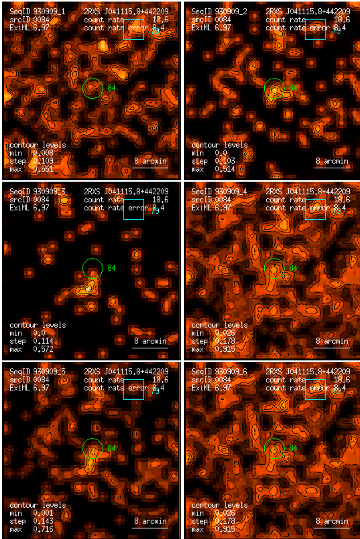
Figure 84: RASS 930909: detection 0084: band rate images, Gaussian filter: (1) PSPC channels 11 – 41, (2) 52 – 90, (3) 91 – 201, (4) 11 – 235, (5) 52 – 201, (6) 11 – 201. Broad band rates in counts/ks. Band rate contour levels in counts/ks/arcmin 2 .
