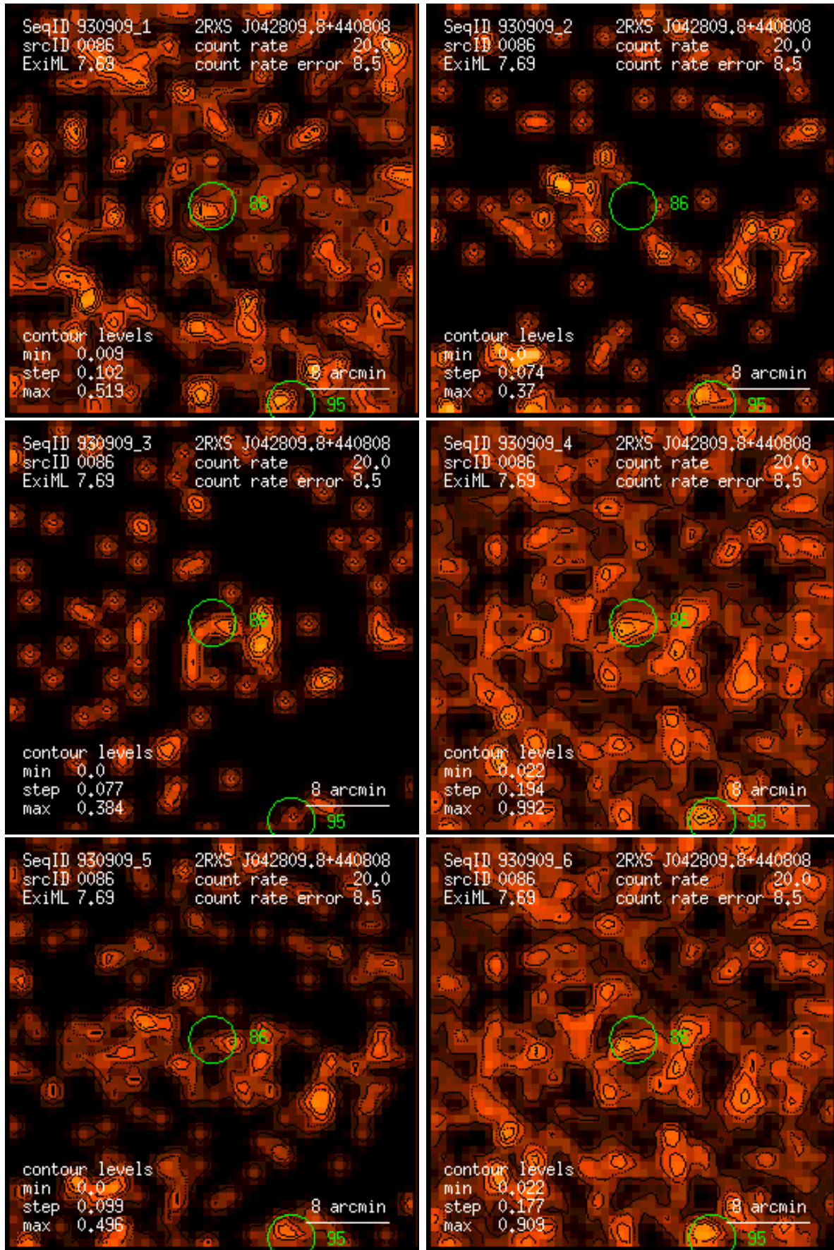
Figure 86: RASS 930909: detection 0086: band rate images, Gaussian filter: (1) PSPC channels 11 – 41, (2) 52 – 90, (3) 91 – 201, (4) 11 – 235, (5) 52 – 201, (6) 11 – 201. Broad band rates in counts/ks. Band rate contour levels in counts/ks/arcmin 2 .
