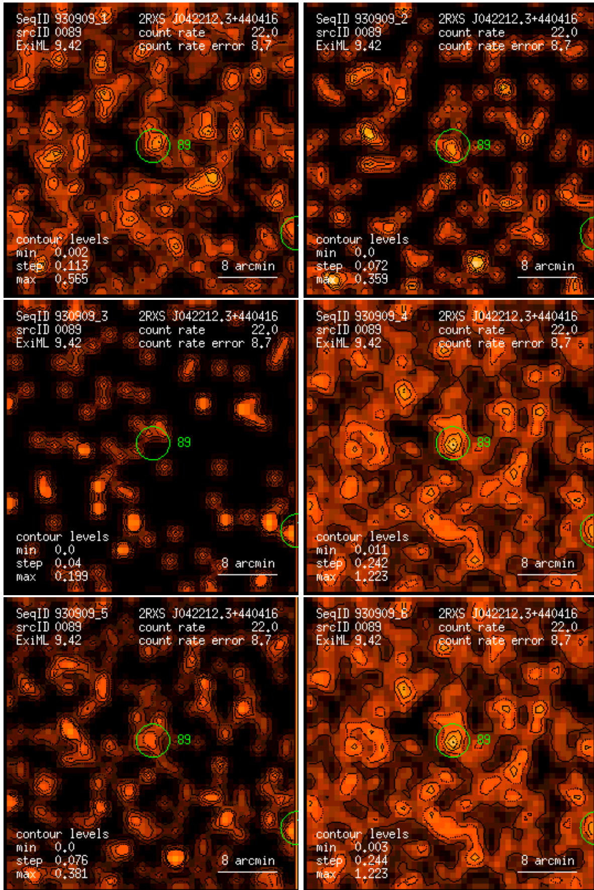
Figure 89: RASS 930909: detection 0089: band rate images, Gaussian filter: (1) PSPC channels 11 – 41, (2) 52 – 90, (3) 91 – 201, (4) 11 – 235, (5) 52 – 201, (6) 11 – 201. Broad band rates in counts/ks. Band rate contour levels in counts/ks/arcmin 2 .
