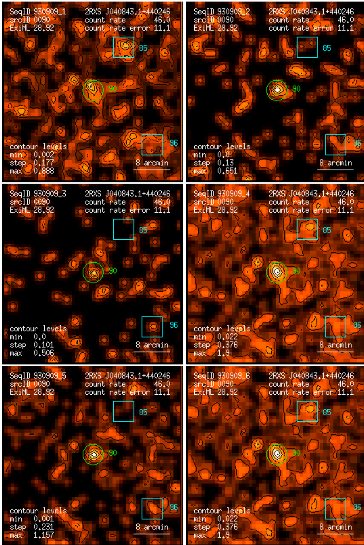
Figure 90: RASS 930909: detection 0090: band rate images, Gaussian filter: (1) PSPC channels 11 – 41, (2) 52 – 90, (3) 91 – 201, (4) 11 – 235, (5) 52 – 201, (6) 11 – 201. Broad band rates in counts/ks. Band rate contour levels in counts/ks/arcmin 2 .
