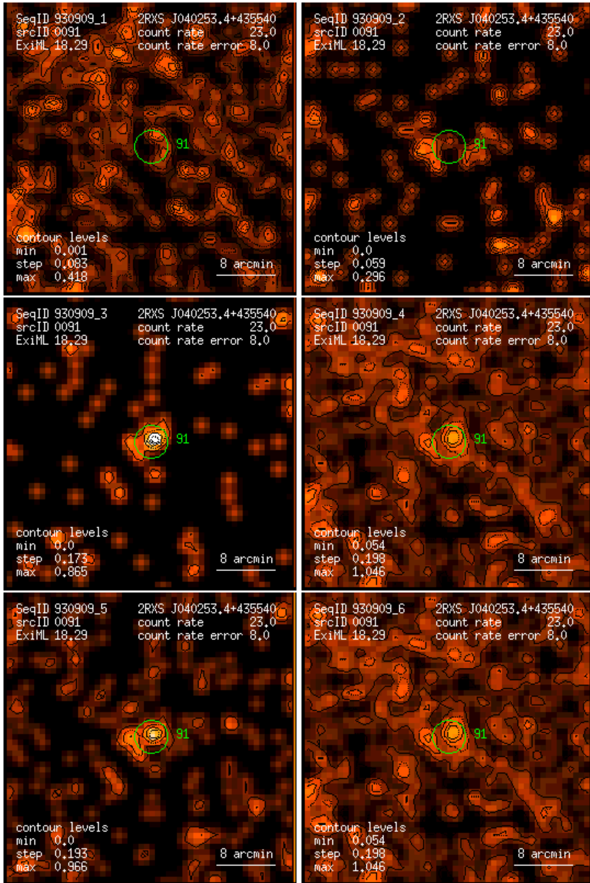
Figure 91: RASS 930909: detection 0091: band rate images, Gaussian filter: (1) PSPC channels 11 – 41, (2) 52 – 90, (3) 91 – 201, (4) 11 – 235, (5) 52 – 201, (6) 11 – 201. Broad band rates in counts/ks. Band rate contour levels in counts/ks/arcmin 2 .
