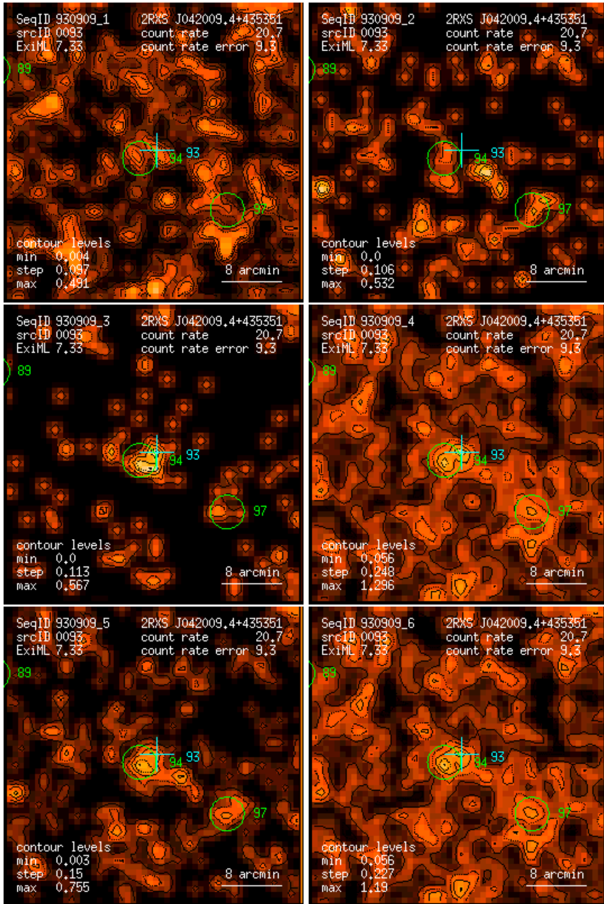
Figure 93: RASS 930909: detection 0093: band rate images, Gaussian filter: (1) PSPC channels 11 – 41, (2) 52 – 90, (3) 91 – 201, (4) 11 – 235, (5) 52 – 201, (6) 11 – 201. Broad band rates in counts/ks. Band rate contour levels in counts/ks/arcmin 2 .
