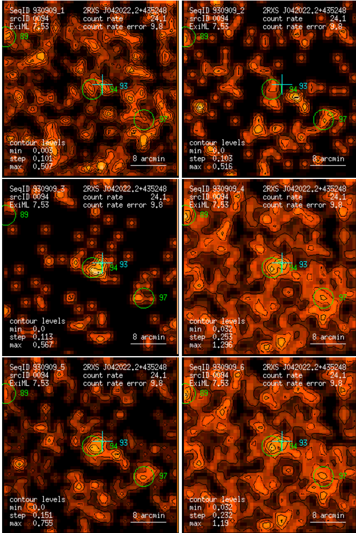
Figure 94: RASS 930909: detection 0094: band rate images, Gaussian filter: (1) PSPC channels 11 – 41, (2) 52 – 90, (3) 91 – 201, (4) 11 – 235, (5) 52 – 201, (6) 11 – 201. Broad band rates in counts/ks. Band rate contour levels in counts/ks/arcmin 2 .
