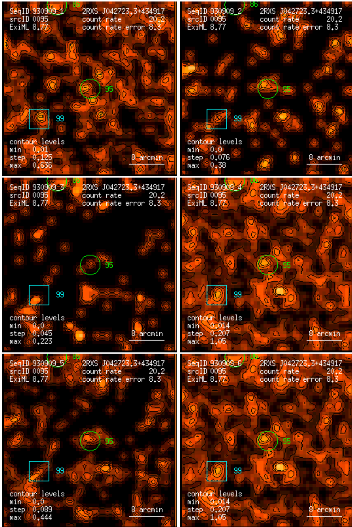
Figure 95: RASS 930909: detection 0095: band rate images, Gaussian filter: (1) PSPC channels 11 – 41, (2) 52 – 90, (3) 91 – 201, (4) 11 – 235, (5) 52 – 201, (6) 11 – 201. Broad band rates in counts/ks. Band rate contour levels in counts/ks/arcmin 2 .
