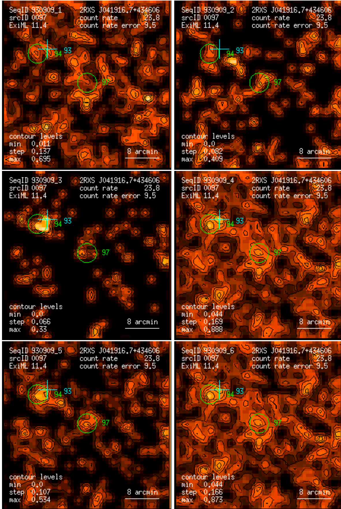
Figure 97: RASS 930909: detection 0097: band rate images, Gaussian filter: (1) PSPC channels 11 – 41, (2) 52 – 90, (3) 91 – 201, (4) 11 – 235, (5) 52 – 201, (6) 11 – 201. Broad band rates in counts/ks. Band rate contour levels in counts/ks/arcmin 2 .
