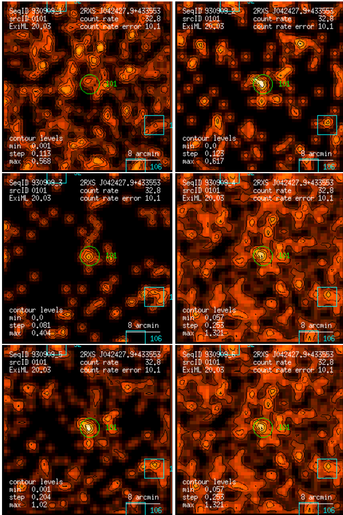
Figure 101: RASS 930909: detection 0101: band rate images, Gaussian filter: (1) PSPC channels 11 – 41, (2) 52 – 90, (3) 91 – 201, (4) 11 – 235, (5) 52 – 201, (6) 11 – 201. Broad band rates in counts/ks. Band rate contour levels in counts/ks/arcmin 2 .
