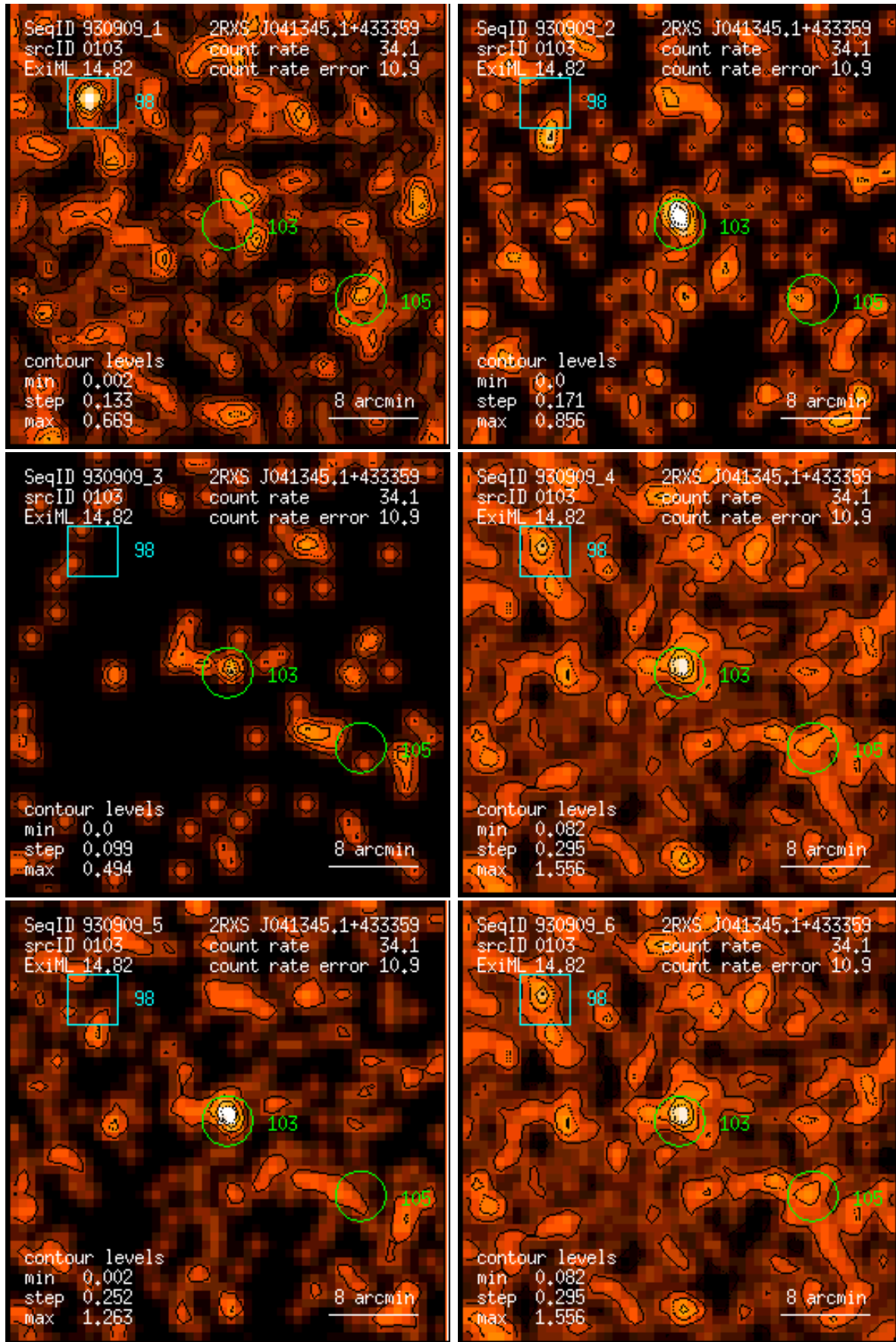
Figure 103: RASS 930909: detection 0103: band rate images, Gaussian filter: (1) PSPC channels 11 – 41, (2) 52 – 90, (3) 91 – 201, (4) 11 – 235, (5) 52 – 201, (6) 11 – 201. Broad band rates in counts/ks. Band rate contour levels in counts/ks/arcmin 2 .
