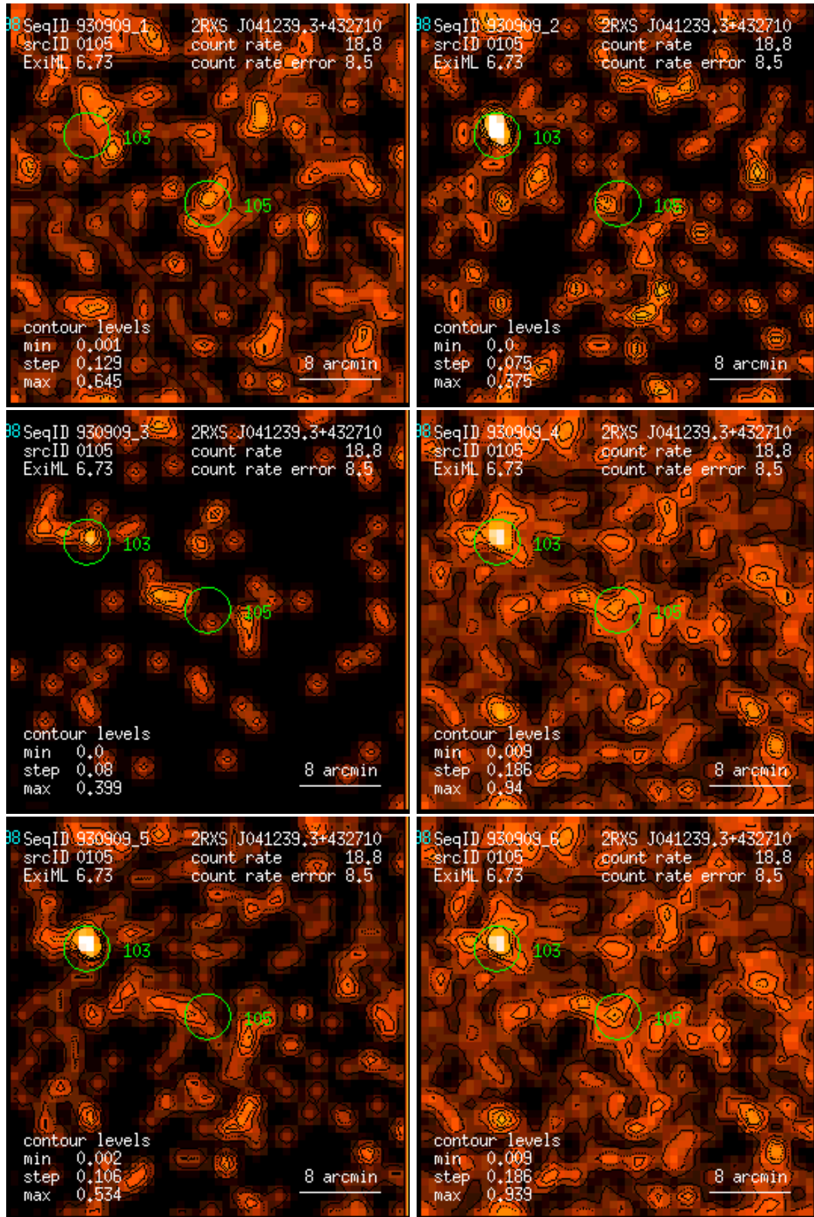
Figure 105: RASS 930909: detection 0105: band rate images, Gaussian filter: (1) PSPC channels 11 – 41, (2) 52 – 90, (3) 91 – 201, (4) 11 – 235, (5) 52 – 201, (6) 11 – 201. Broad band rates in counts/ks. Band rate contour levels in counts/ks/arcmin 2 .
