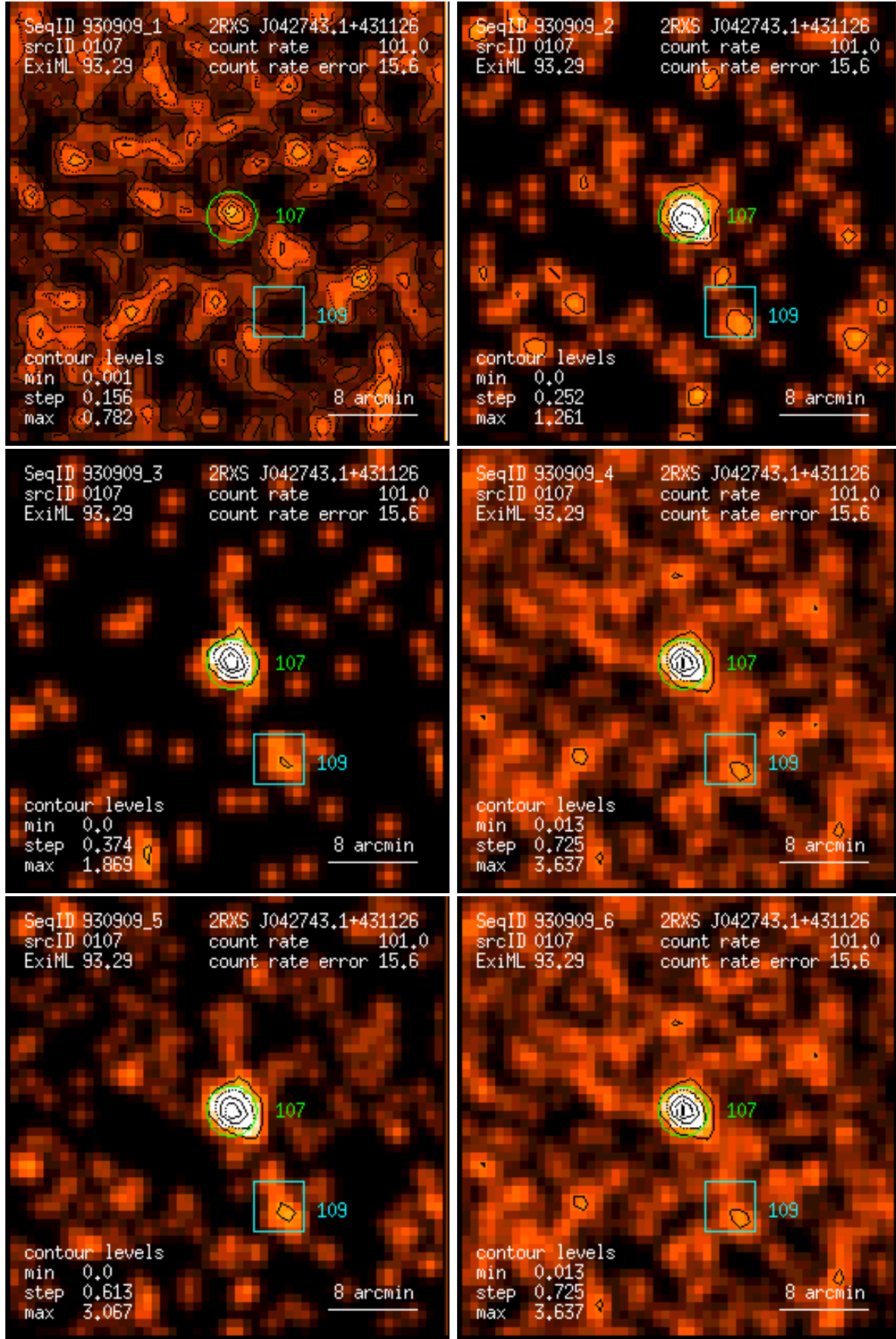
Figure 107: RASS 930909: detection 0107: band rate images, Gaussian filter: (1) PSPC channels 11 – 41, (2) 52 – 90, (3) 91 – 201, (4) 11 – 235, (5) 52 – 201, (6) 11 – 201. Broad band rates in counts/ks. Band rate contour levels in counts/ks/arcmin 2 .
