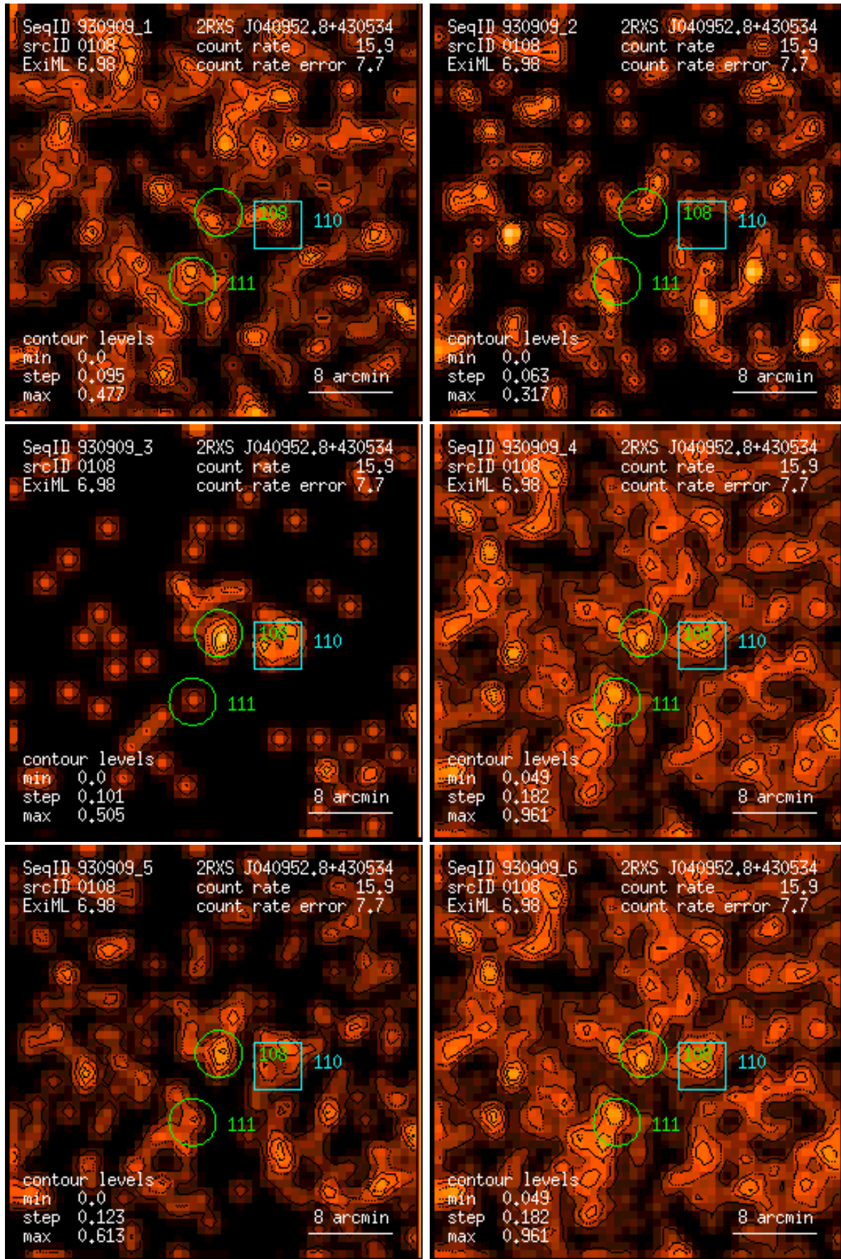
Figure 108: RASS 930909: detection 0108: band rate images, Gaussian filter: (1) PSPC channels 11 – 41, (2) 52 – 90, (3) 91 – 201, (4) 11 – 235, (5) 52 – 201, (6) 11 – 201. Broad band rates in counts/ks. Band rate contour levels in counts/ks/arcmin 2 .
