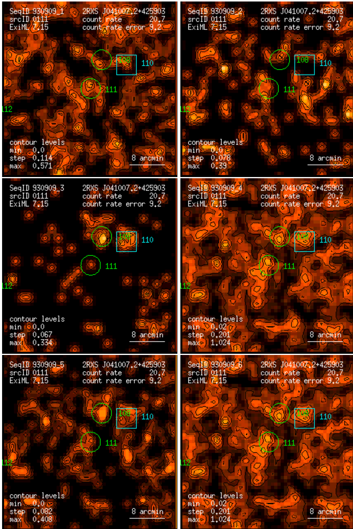
Figure 111: RASS 930909: detection 0111: band rate images, Gaussian filter: (1) PSPC channels 11 – 41, (2) 52 – 90, (3) 91 – 201, (4) 11 – 235, (5) 52 – 201, (6) 11 – 201. Broad band rates in counts/ks. Band rate contour levels in counts/ks/arcmin 2 .
