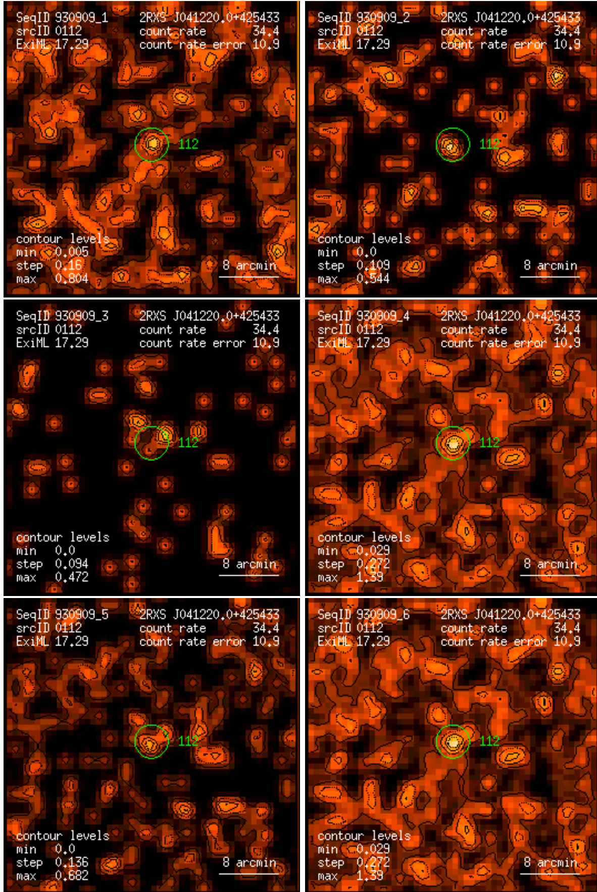
Figure 112: RASS 930909: detection 0112: band rate images, Gaussian filter: (1) PSPC channels 11 – 41, (2) 52 – 90, (3) 91 – 201, (4) 11 – 235, (5) 52 – 201, (6) 11 – 201. Broad band rates in counts/ks. Band rate contour levels in counts/ks/arcmin 2 .
