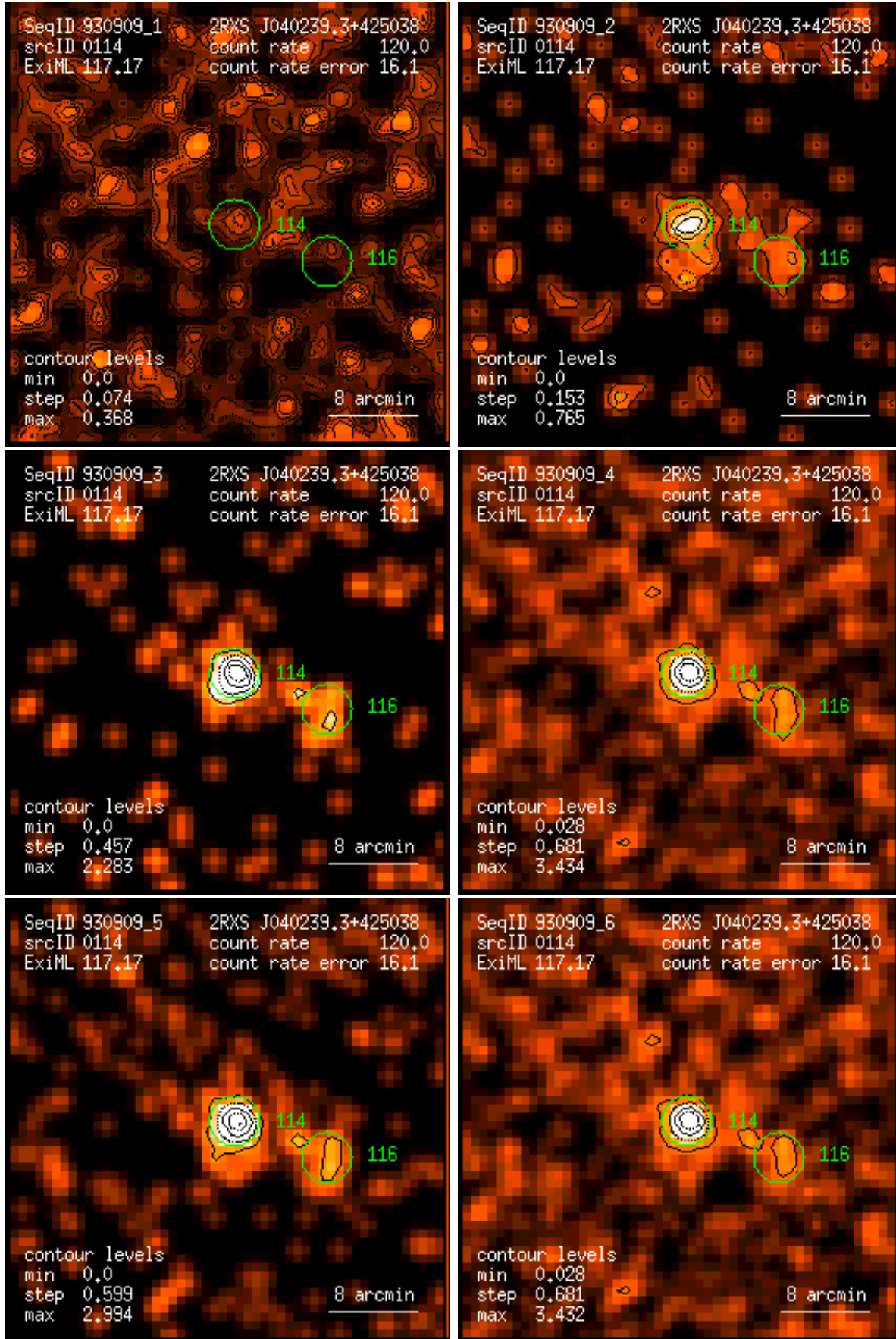
Figure 114: RASS 930909: detection 0114: band rate images, Gaussian filter: (1) PSPC channels 11 – 41, (2) 52 – 90, (3) 91 – 201, (4) 11 – 235, (5) 52 – 201, (6) 11 – 201. Broad band rates in counts/ks. Band rate contour levels in counts/ks/arcmin 2 .
